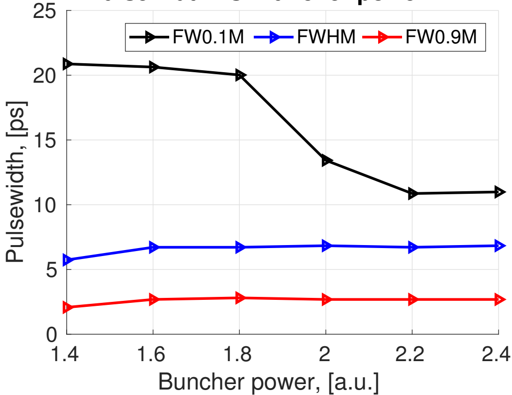
Pulsewidth vs. Buncher power
