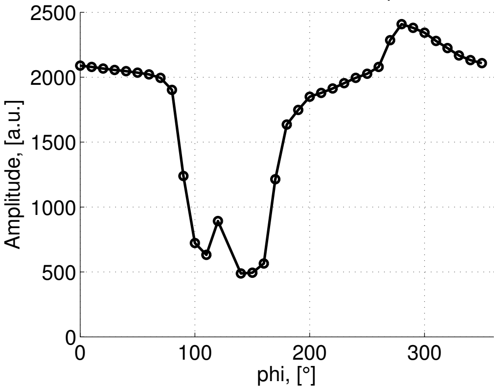
Maximum of convolution with 15ps window
