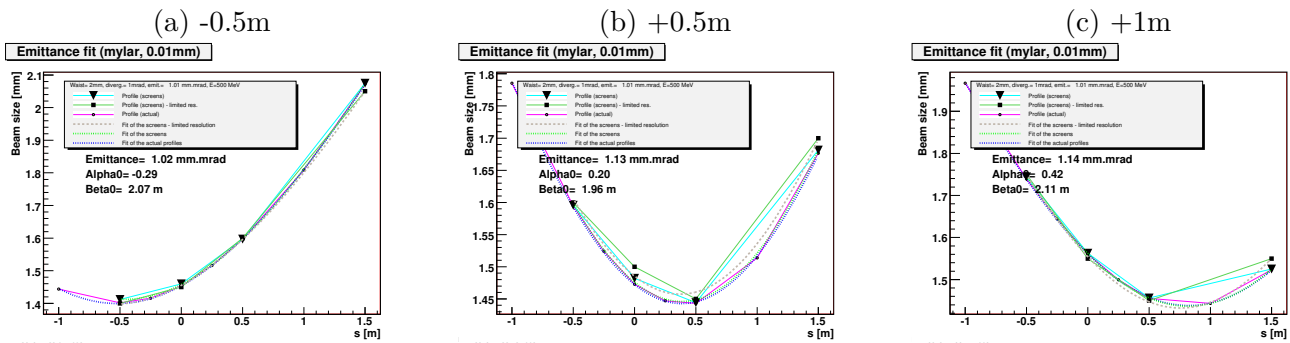
Figure 1.16: Scattering induced in a 500 MeV for 10\mu\text{m} -thick Mylar screens for a 500 MeV beam with an initial emittance of 1mm.mrad when the waist is not located on the second screen. The waist position is given above the plot. The black squares show the beam size observed on each screen, the black triangles show the beam size rounded to the nearest 50\mu\text{m} (to simulate what is observed by a camera with a limited pixel size). The open circles are the position measured at additional intermediate positions. The dashed brown line shows the emittance fit made using the black triangles. The dashed green line shows the emittance fit made using the black square. The dashed green line shows the emittance fit made using the open circles. The values given on the plot below the legend for the emittance, \alpha_0 and \beta_0 are those extracted from the fit on the beam sizes with limited pixel size.
