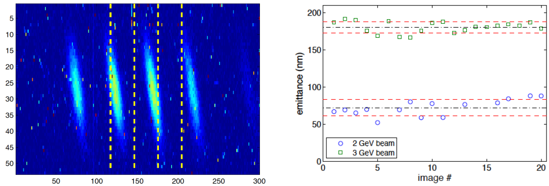
Figure 1.6: Pepper pot measurement at the DIAMOND Light Source as reported in the booster to synchrotron line with a beam energy of 2 GeV and 3 GeV. Left: image recorded by the camera. Right: transverse emittance calculated shot by shot on several images. Images taken from [?].
