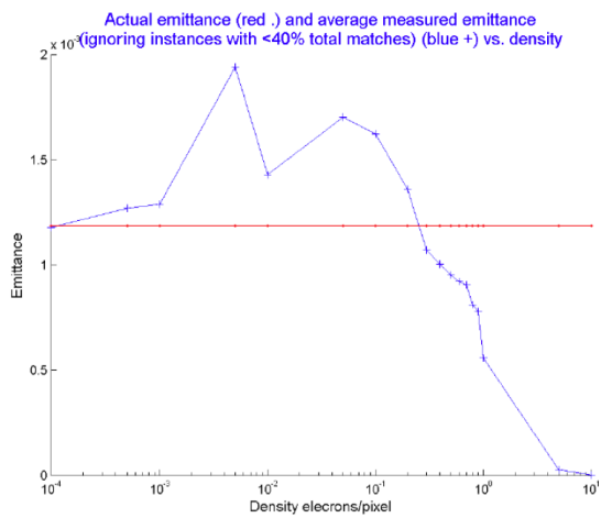
Figure 1.24: Accuracy of the emittance reconstruction depending on the electrons density (simulations taken from [?]).
