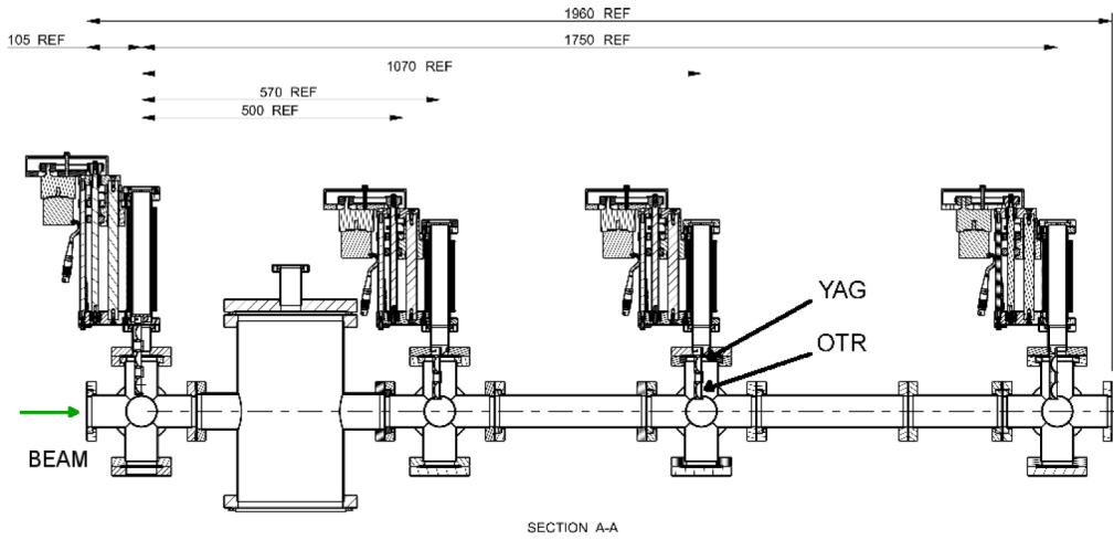
Figure 1.19: Drawing of the multiple OTR and pepper-pot test beam line that has been used both at Frascati's Beam Test Facility and at the Diamond Light Source. Image taken from [?].
