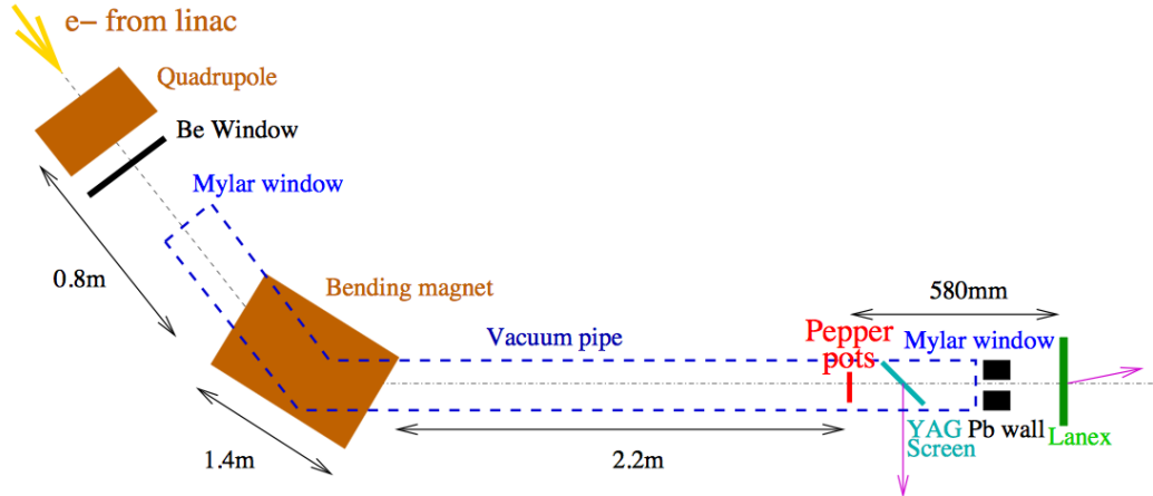
Figure 1.3: Layout of the pepper-pot experiment at the BTF as shown in [?].
