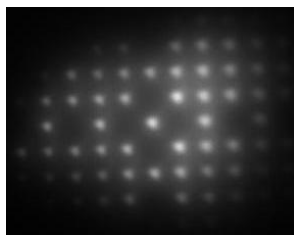
Figure 1.2: Example of pepper-pot measurement using the Oxford teaching accelerator (image taken from [?]).
