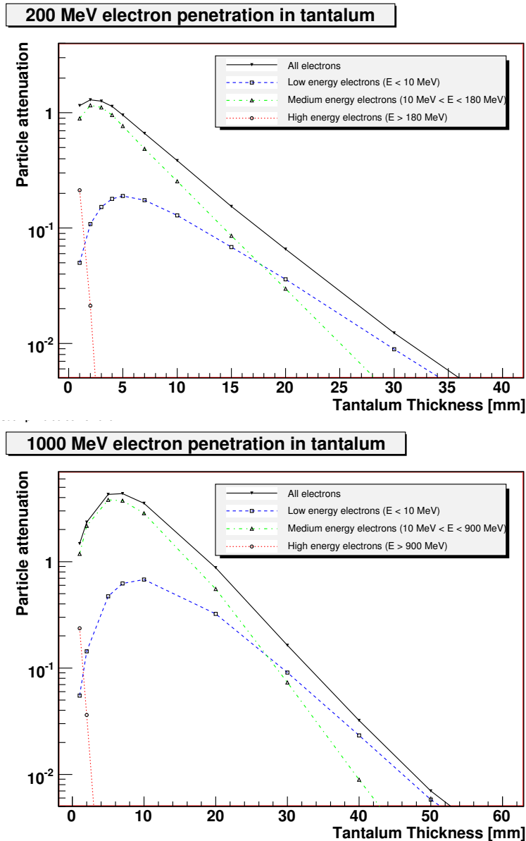
Figure 1.7: GEANT4 [?] simulations of the penetration of high energy electrons in a block of Tantalum. The horizontal axis gives the penetration depth and the vertical axis gives the number of electrons remaining at that depth for one initial electron. The red lines (round markers) correspond to high energy electrons whereas the blue lines (square markers) and the green lines (up-pointing triangular markers) correspond to lower energy particles emitted by the initial particle. The black lines (down-pointing triangular markers) show the total number of electrons remaining. The plot on the top corresponds to 200 MeV electrons and the one on the bottom to 1 GeV electrons. Figure taken from [?].
