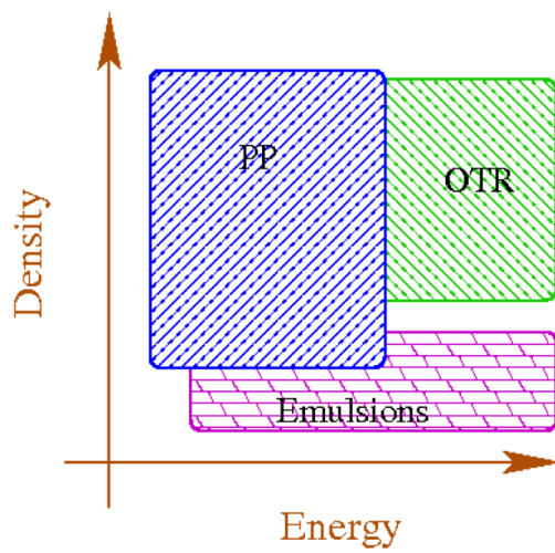
Figure 1.27: Range of applicability of the three techniques discussed in this chapter: the emulsions are better suited to low density beams; the pepper-pots are better suited to high density beams and rather low energy (up to a few GeV) whereas the OTR techniques are better suited to high intensity high energy beam..
