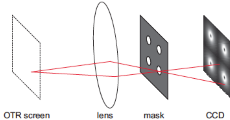
Figure 1.25: Layout of the masked OTR setup as taken from [?].
