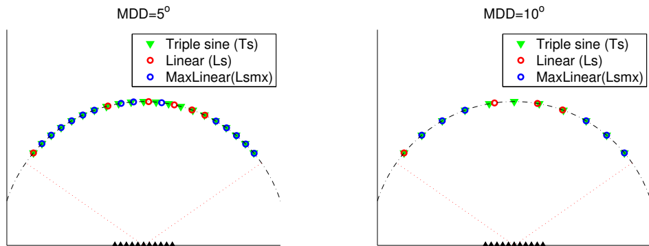
Figure 1.17: Examples of detector positions for different types of sampling for a minimal detector distance of 5^\circ (left) and 10^\circ (right), as presented in [54].
