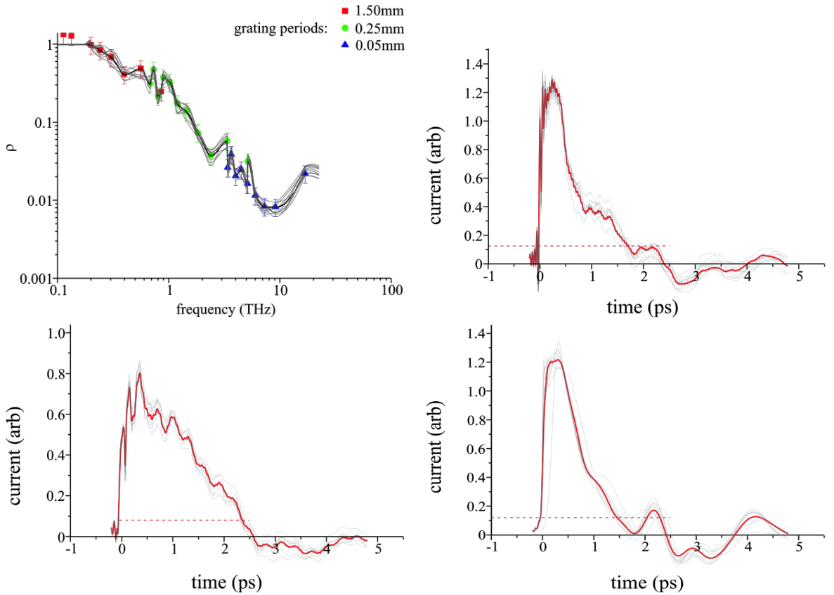
Figure 1.21: Top left: The magnitude of the Fourier Transform of the time profile of the bunch for a ?high compression? run on the 9 April 2013 (see text in [43]). Other plots: bunch profile reconstructed from measurements at different times and with different bunch compression settings (top right: 9 April 2013, high compression; bottom left: 9 April 2013, medium compression; bottom right: 25 June 2013). Plots taken from [43] where more explanations can be found.
