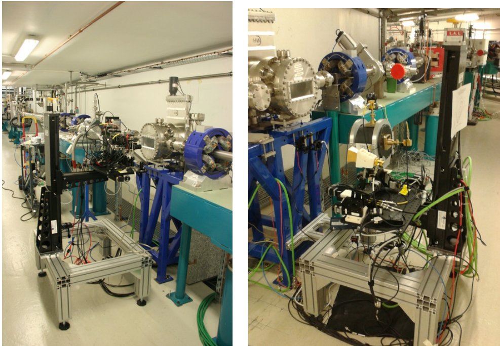
Figure 1.24: The experimental setup of SPESO at the end of the SOLEIL Linac: left, as it was in 2015 (image taken from [58]) and right with the polarizer installed in 2016 (image taken from [59]). On both images the electrons travels from left to right.
