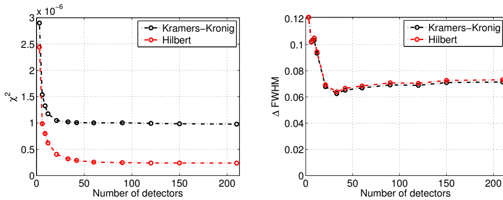
Figure 1.15: Effect of the sampling frequencies (number of detectors) on the \chi^2 (left) and \Delta_{FWHM} (right) when comparing original and reconstructed profiles, as presented in [54].
