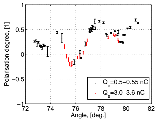
Figure 1.27: Degree of polarisation as function of the longitudinal displacement (along the beam propagation axis). Image taken from [59].
