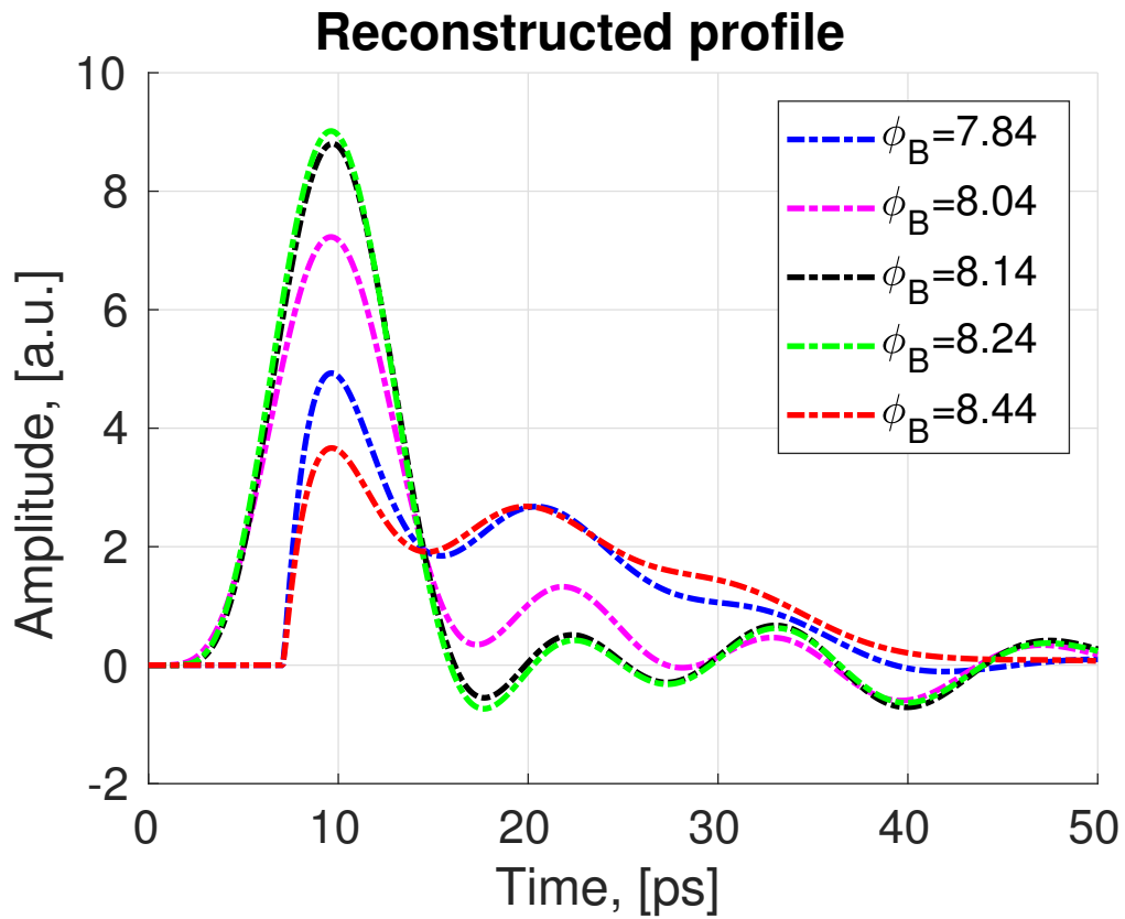
Figure 1.33: Bunche profile reconstructed on CLIO for different buncher phase as reported in [67].
