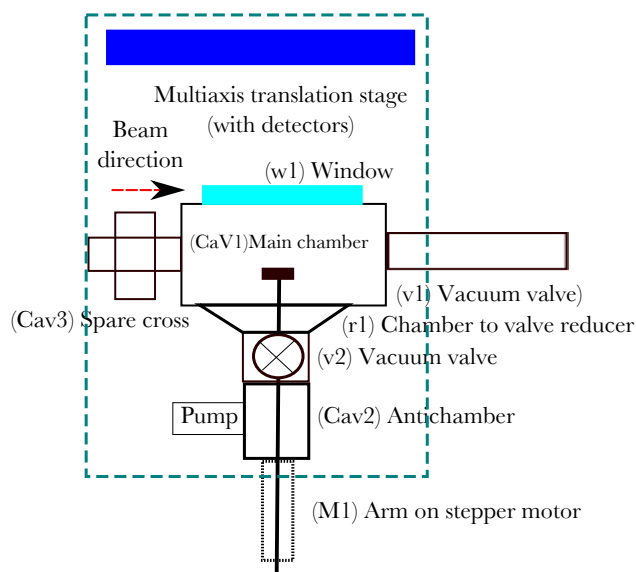
Figure 1.23: The experimental setup of SPESO at the end of the SOLEIL Linac (image taken from [58]).
