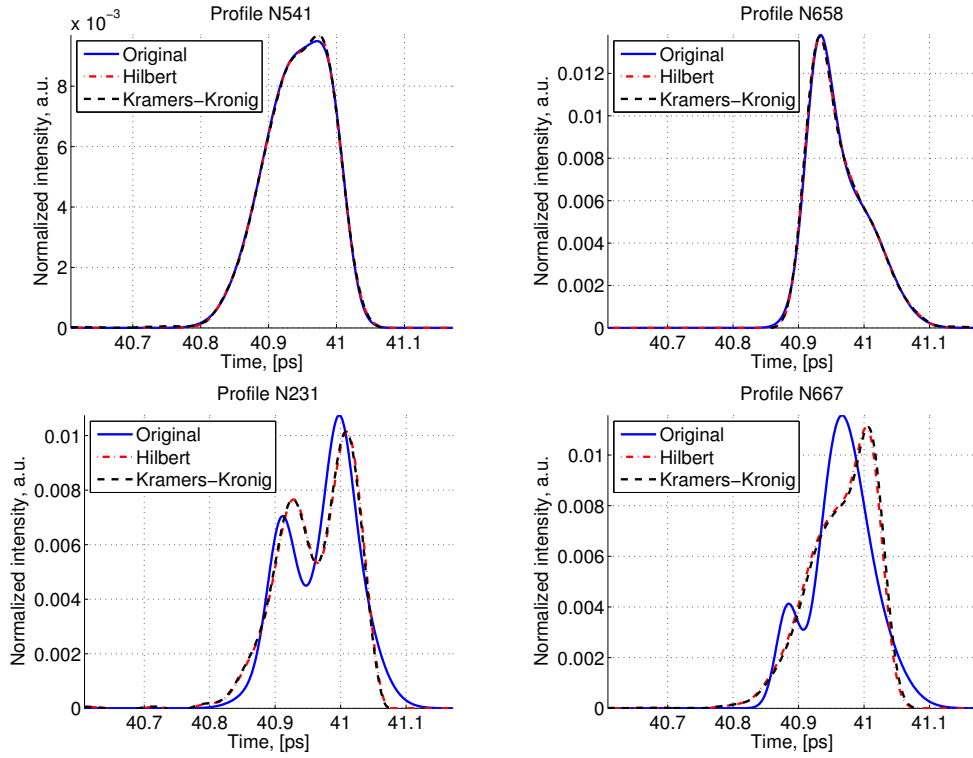
Figure 1.14: Example of profiles correctly reconstructed (upper row) and poorly reconstructed (lower row) as presented in [54]. The original profile is in blue and the profiles reconstructed with the Hilbert transform and the full Kramers-Kronig procedures are in red and black respectively.
