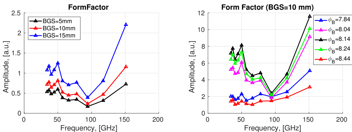
Figure 1.32: Form factor measured at CLIO as reported in [67]. Left: Variation of the form factor when the beam grating separation varies. Right: Variation of the form factor when the buncher phase varies.
