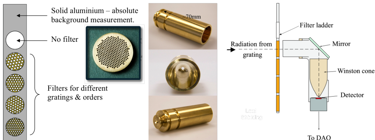
Figure 1.20: The optical parts of the E-203 experiment: (from left to right) the filters, the optical concentrators (winston cones) and the optical assembly (image taken from [43]).
