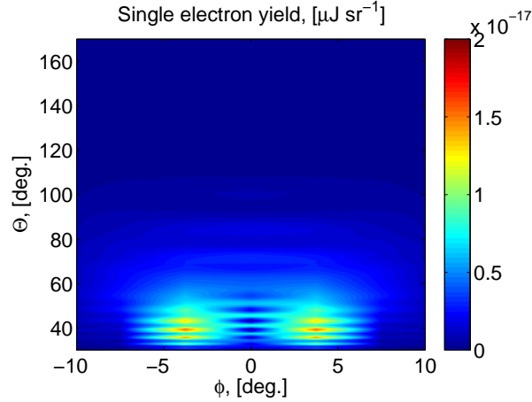
Figure 1.11: Single electron yield of Smith-Purcell radiation for a 40 \times 180 mm 2 grating with a 8 mm pitch and a 30^\circ blaze angle. Image taken from [46].
