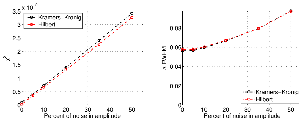
Figure 1.18: Mean \chi^2 and \Delta_{FWXM} as function of the noise amplitude, as presented in [54]. The interpretation of this figure is that with a 50% noise on our signal we introduce an error on the profile FWHM of about 10%.
