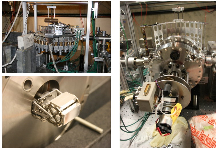
Figure 1.19: The E-203 experiment (during pre-installation tests) seen from the detectors side (top left), from the motors side (right) and the grating's carousel (bottom left). Images taken from [42].
