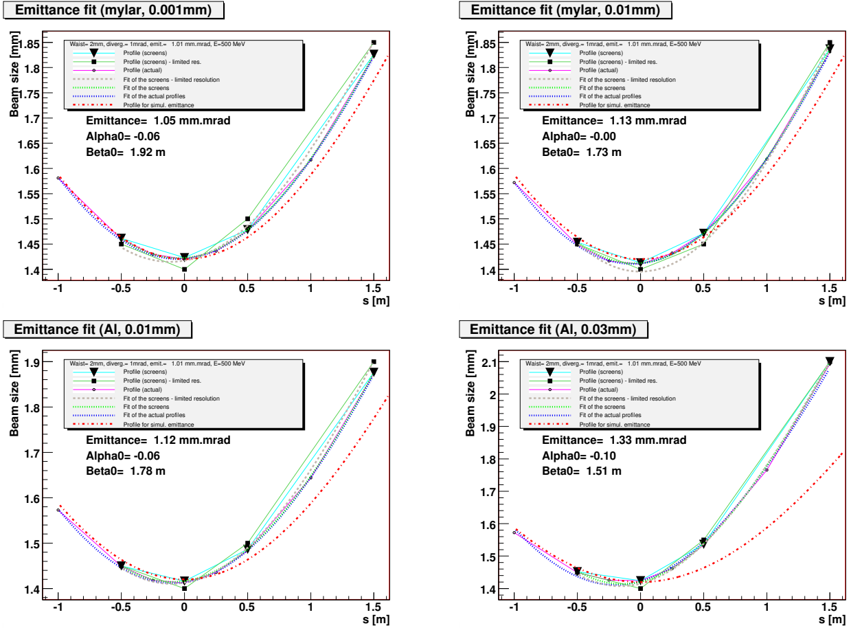
Figure 1.16: Scattering induced in a 500 MeV for various screen material and thickness with an initial emittance of 1mm.mrad. The screens material and thickness is given in the plot title. The black squares show the beam size observed on each screen, the black triangles show the beam size rounded to the nearest 50 \mu\text{m} (to simulate what is observed by a camera with a limited pixel size). The open circles are the position measured at additional intermediate positions. The dashed brown line shows the emittance fit made using the black triangles. The dashed green line shows the emittance fit made using the black square. The dashed green line shows the emittance fit made using the open circles. The dashed red line is the theoretical profile of the beam assuming \alpha_0 = 0 , \beta_0 = 2.0\text{m} and \epsilon = 1.01\text{mm.mrad} . The values given on the plot below the legend for the emittance, \alpha_0 and \beta_0 are those extracted from the fit on the beam sizes with limited pixel size.
