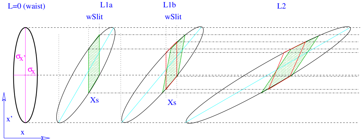
Figure 1.9: Long pepper-pot: Evolution of the phase-space as the beam drifts. At the source or at a waist ( L = 0 ) the phase space of the beam is first represented by an upright ellipse. As the beam drifts the ellipse gets sheared. At L_{1a} the beam enters a slit and thus only the particles in the green area pass the slit. While the beam travels in the slit the ellipse is further sheared, hence at L_{1b} , the exit of the slit, the area of phase space within the slit acceptance (red box) is different from that occupied by the particles sampled at the entrance of the slit. Hence the full acceptance of the slit correspond to the overlap between the green and the red areas. Figure taken from [?]. The variables definition is given in [?].
