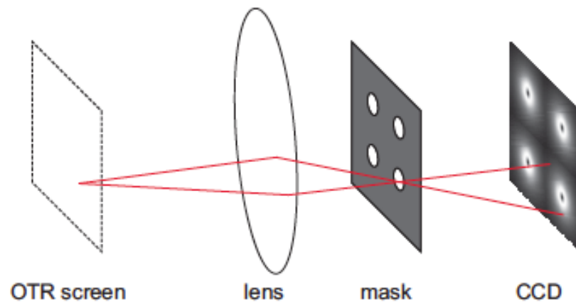
Figure 1.26: Layout of the masked OTR setup as taken from [?].
