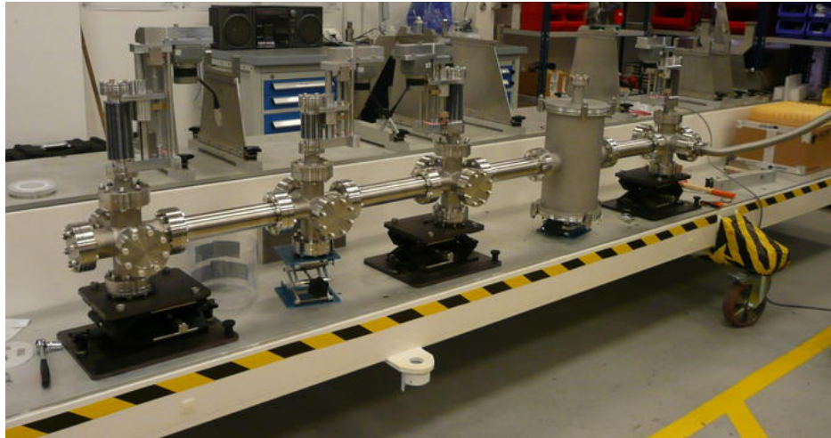
Figure 1.19: The multiple OTR and pepper-pot test beam line during a test installation at the Diamond Light Source before its shipment to Frascati.
