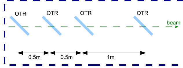
Figure 1.11: Screen layout used in the calculations of multiple OTR single shot emittance measurement.
