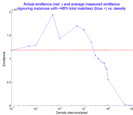
Figure 1.25: Accuracy of the emittance reconstruction depending on the electrons density (simulations taken from [?]).
