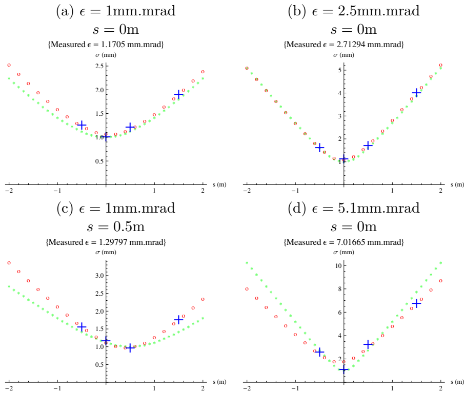
Figure 1.12: Simulated (small green dots), measured (blue crosses) and fitted (red circles) beam sizes ( \sigma ) around the waist. The beam transverse emittance ( \epsilon ) and waist offset ( s ) is indicated above each plot. The waist size is always assumed to be 1 mm and the pixel size 20\mu\text{m} . The screens used are assumed to satisfy equation 7.13 and thus the effect of the scattering is neglected in these plots.
