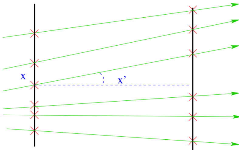
Figure 1.24: Emittance measurement using nuclear emulsions tracking.
