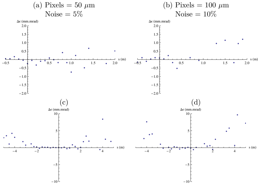
Figure 1.14: Error on the emittance measurement as a function of the position of the beam waist for beams with an emittance of 1 mm.mrad forming a 1 mm waist at the indicated position. In plot (a) and (c) the pixel size is 50 \mu\text{m} and the noise is 5%. In plot (b) and (d) the pixel size is 100 \mu\text{m} and the noise is 10%. Plot (c) and (d) repeat plot (a) and (b) over a longer range. The screens used are assumed to satisfy equation 7.13 and thus the effect of the scattering is neglected in these plots.
