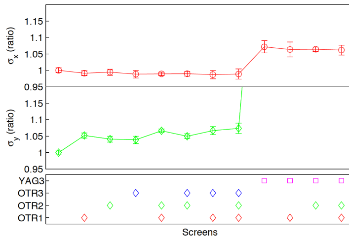
Figure 1.21: Beam size on the fourth OTR screen during the Diamond Tests as function of the screens inserted upstream. We can see that the effect of the upstream screens on the beam size measured on the lat screen is negligible in x and about 5% in y as was expected from our calculations. Image taken from [?].
