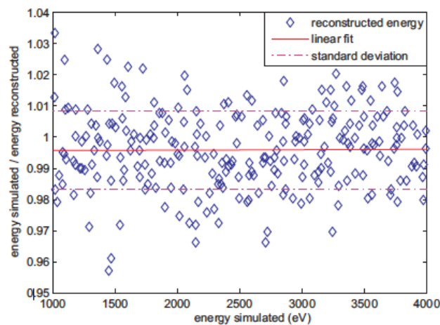
Figure 1.27: Simulations of energy measurements using masked OTR taken from [?].
