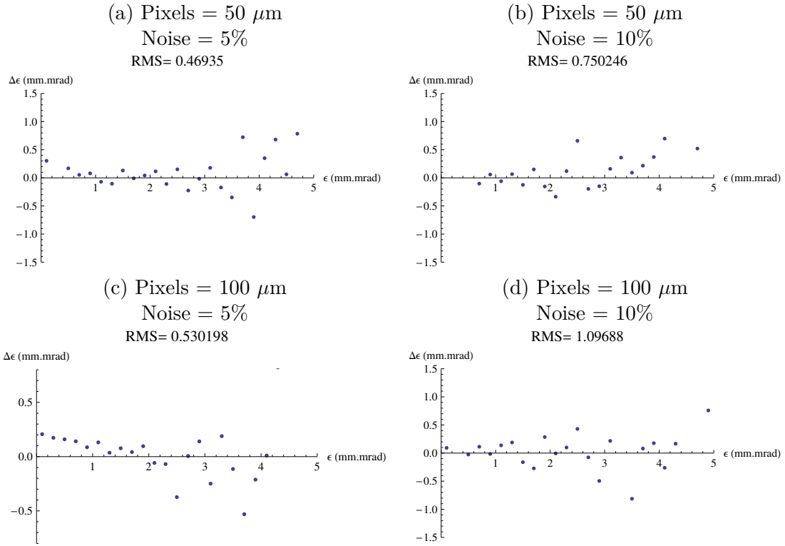
Figure 1.13: Error on the emittance measurement as a function of the beam emittance for beams forming a 1 mm waist at s = 0 . In plots (a) and (b) the pixel size is 50 \mu\text{m} and in plots (c) and (d) it is 100 \mu\text{m} . For plot (a) and (c) the error on the beam size measurement is 5%, for plot (b) and (d) it is 10%. The screens used are assumed to satisfy equation 7.13 and thus the effect of the scattering is neglected in these plots.
