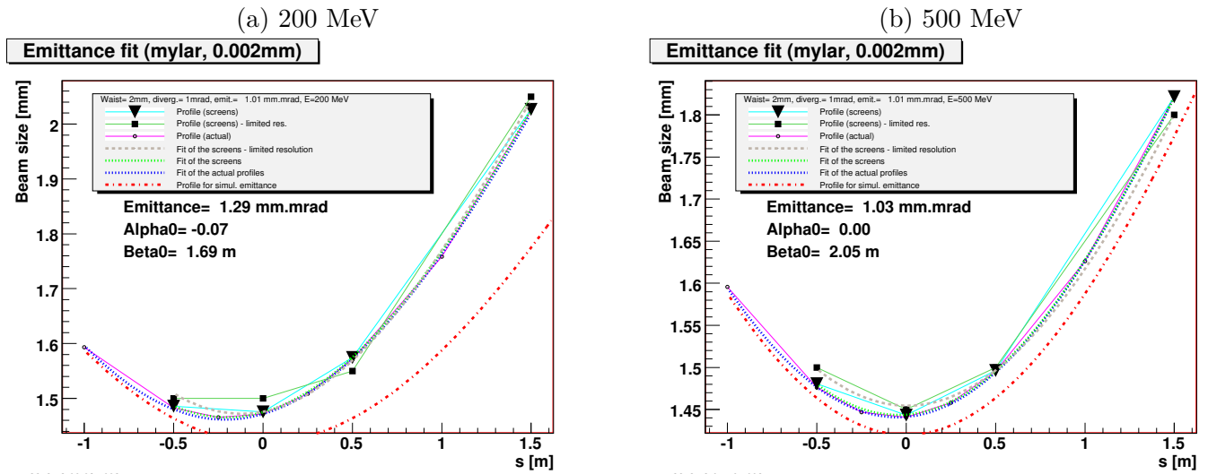
Figure 1.18: Emittance fit using 2\mu\text{m} -thick Mylar screens at 200 MeV (a) and 500 MeV (b). The black squares show the beam size observed on each screen, the black triangles show the beam size rounded to the nearest 50\ \mu\text{m} (to simulate what is observed by a camera with a limited pixel size). The open circles are the position measured at additional intermediate positions. The dashed brown line shows the emittance fit made using the black triangles. The dashed green line shows the emittance fit made using the black square. The dashed green line shows the emittance fit made using the open circles. The dashed red line is the theoretical profile of the beam assuming \alpha_0 = 0 , \beta_0 = 2.0\text{m} and \epsilon = 1.01\text{mm.mrad} . The values given on the plot below the legend for the emittance, \alpha_0 and \beta_0 are those extracted from the fit on the beam sizes with limited pixel size.
