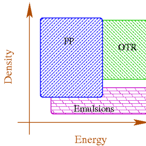
Figure 1.28: Range of applicability of the three techniques discussed in this chapter: the emulsions are better suited to low density beams; the pepper-pots are better suited to high density beams and rather low energy (up to a few GeV) whereas the OTR techniques are better suited to high intensity high energy beam..
