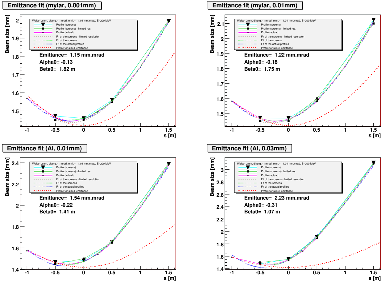
Figure 1.15: Scattering induced in a 200 MeV for various screen material and thickness with an initial emittance of 1mm.mrad. The screens material and thickness is given in the plot title. The black squares show the beam size observed on each screen, the black triangles show the beam size rounded to the nearest 50 \mu m (to simulate what is observed by a camera with a limited pixel size). The open circles are the position measured at additional intermediate positions. The dashed brown line shows the emittance fit made using the black triangles. The dashed green line shows the emittance fit made using the black square. The dashed green line shows the emittance fit made using the open circles. The dashed red line is the theoretical profile of the beam assuming \alpha_0 = 0 , \beta_0 = 2.0m and \epsilon = 1.01mm.mrad . The values given on the plot below the legend for the emittance, \alpha_0 and \beta_0 are those extracted from the fit on the beam sizes with limited pixel size.
