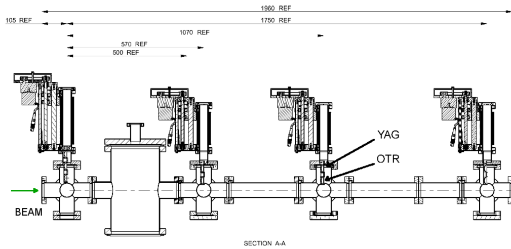
Figure 1.20: Drawing of the multiple OTR and pepper-pot test beam line that has been used both at Frascati's Beam Test Facility and at the Diamond Light Source. Image taken from [?].
