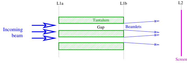
Figure 1.8: Example of a “extended” pepper-pot sampling a beam into several beamlets. The transverse emittance is given by using the hole size and the beamlets divergence measured on the screen (image taken from [?]).
