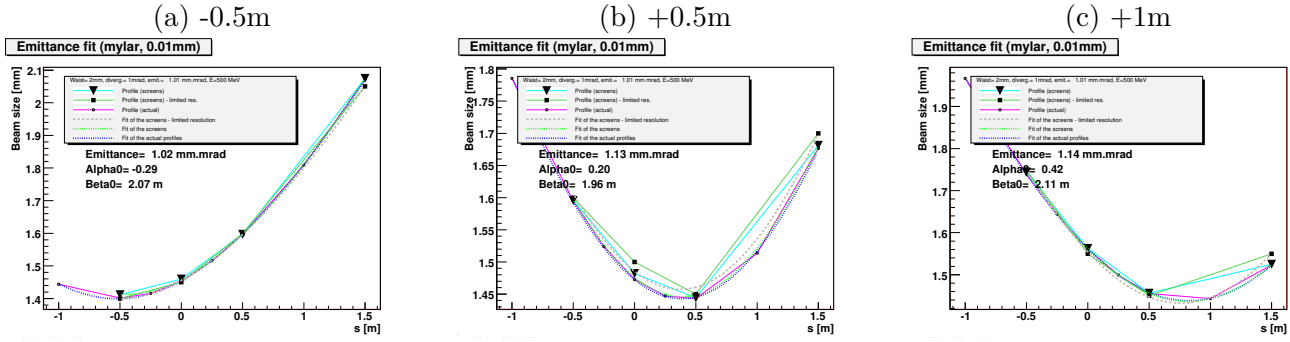
Figure 1.17: Scattering induced in a 500 MeV for 10\mu\text{m} -thick Mylar screens for a 500 MeV beam with an initial emittance of 1mm.mrad when the waist is not located on the second screen. The waist position is given above the plot. The black squares show the beam size observed on each screen, the black triangles show the beam size rounded to the nearest 50\mu\text{m} (to simulate what is observed by a camera with a limited pixel size). The open circles are the position measured at additional intermediate positions. The dashed brown line shows the emittance fit made using the black triangles. The dashed green line shows the emittance fit made using the black square. The dashed green line shows the emittance fit made using the open circles. The values given on the plot below the legend for the emittance, \alpha_0 and \beta_0 are those extracted from the fit on the beam sizes with limited pixel size.
