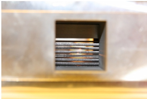
Figure 7.4: Picture of the pepper-pot used at the BTF as shown in [75].
