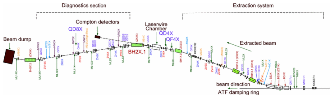
Figure 3.3: Layout of the ATF extraction line showing the location of the laser-wire. Image taken from [44].
