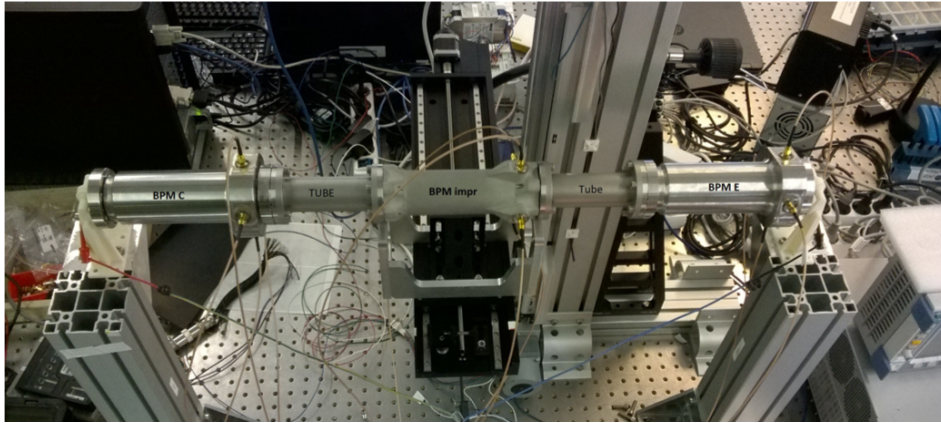
Figure 2: The test bench where the three BPMs have been measured. The BPM built using additive manufacturing is in the middle et the two ones built using conventionnal means are on the ends. Translation stages allow to move the BPMs vertically and horizontally (transverse to the BPM axis). A conducting metallic wire is stretched through the BPMs and electric pulses are sent on it.
