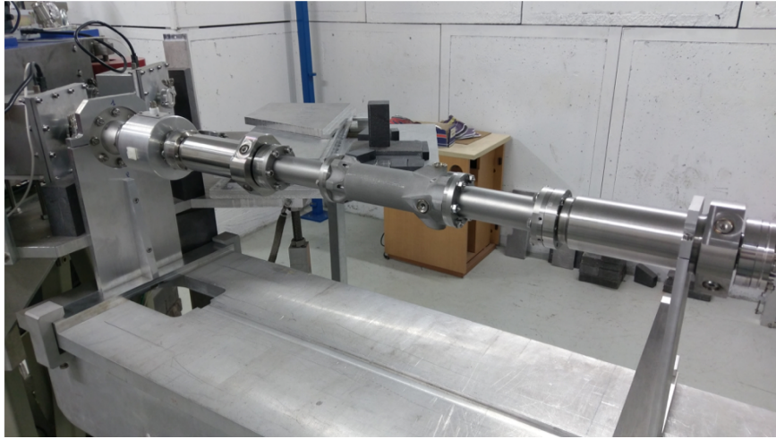
Figure 5: The BPM triplet installed on PHIL. The beam is coming from the left to the right. On the picture one can see (from left to red), first an ICT then one of the conventional BPM, the i3D BPM and the other conventional BPM. There is no magnetic element between the BPMs.
