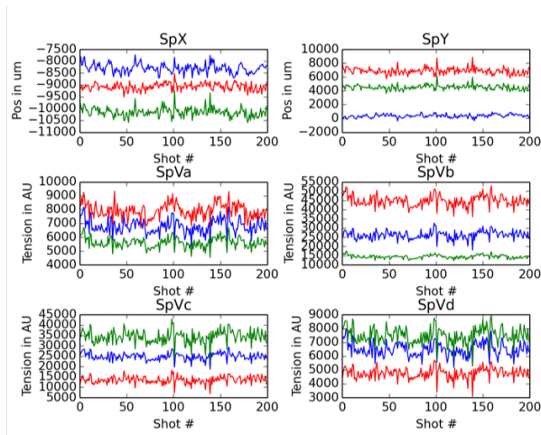
Figure 6: Bottom four plots: Reading by each of the four electrodes (SpVa, SpVb, SpVc and SpVd) of the three BPMs (represented by three colors, red, blue and green, the i3D BPM is in red). Top two plots: X (horizontal) and Y (vertical) position of the beam calculated by the libera. Given that the reading the i3D BPM were higher a factor two higher attenuation was applied to these electrodes. The data were acquired in single pass mode.
