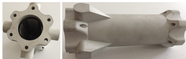
Figure 1: CAD 3D view of the i3D BPM (top) and pictures of the BPM after printing. The shapes have been created by topological optimization. Electrical feedthrough have been added separately.
