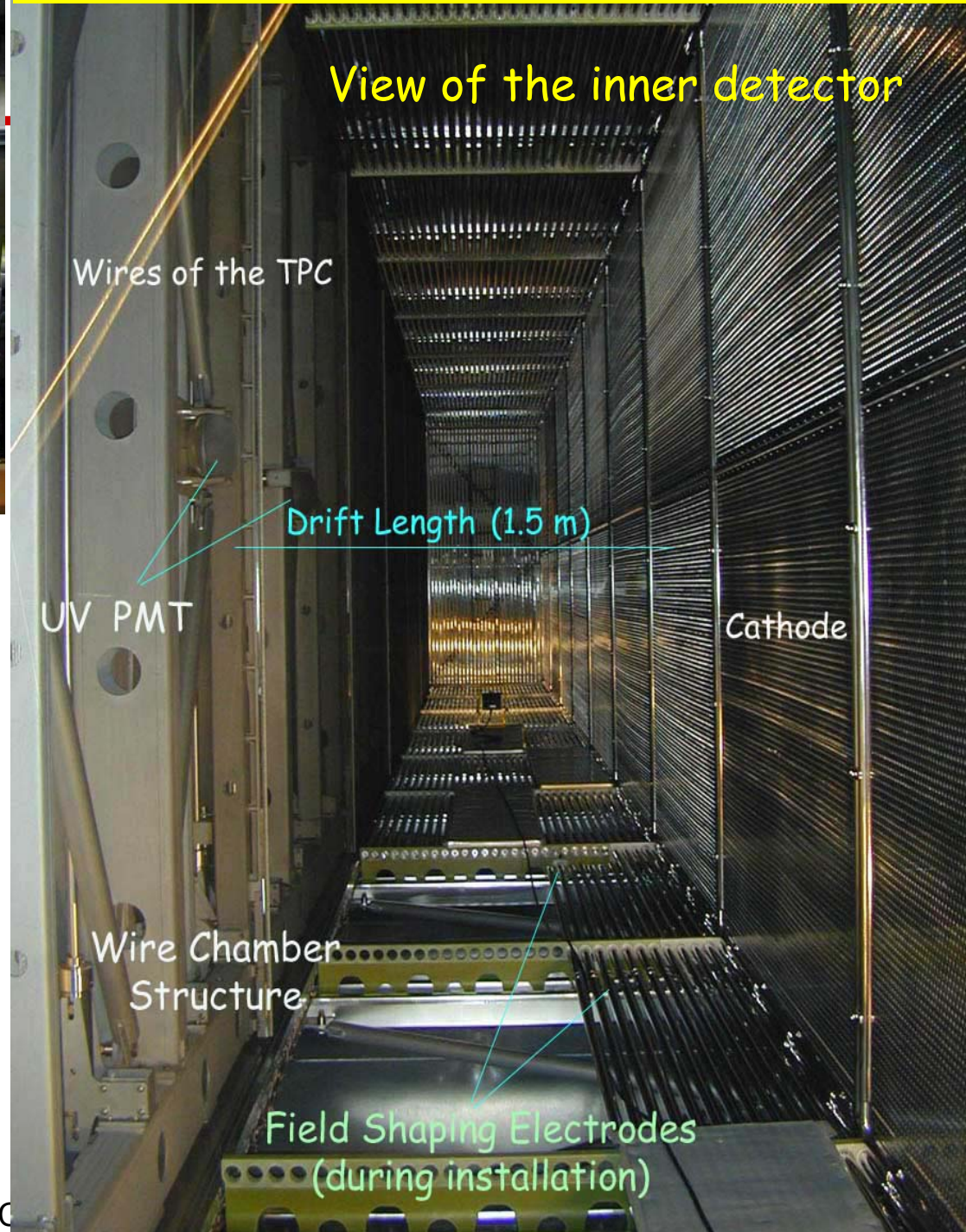
ICARUS T300 prototype
