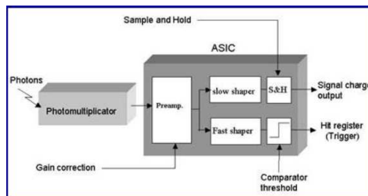
Figure 12: Sketch of the existing Read Out electronics developed for the OPERA Target Tracker and that is intended to be extended for MEMPHYS by integrating the ADC and TDC.
