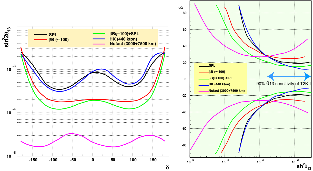
Figure 10: LEFT : \theta_{13} 90% C.L. sensitivity as function of \delta_{CP} for \Delta m_{23}^2 = 2.5 \cdot 10^{-3} eV^2 , \text{sign}(\Delta m_{23}^2) = 1 , 2% systematic errors. SPL-SB sensitivities have been computed for a 2 year \nu_{\mu} + 8 year \bar{\nu}_{\mu} run, \beta B ( \gamma = 100 ) for a 5 year \nu_e + 5 year \bar{\nu}_e run, 200 MeV energy bins for both beams. The combination of SPL-SB and \beta B is also shown. HK and NuFACT curves are adapted from [30]: HK curves corresponds to Hyperkamioka with the same fiducial mass, running time and systematics as MEMPHYS, using the 4MW beam from JAERI. The NuFACT curve corresponds to 5 year runs for each polarity, two 50kton iron detectors located at 3000 and 7000 km receiving neutrinos from 10^{21} useful 50 GeV muon decays per year, detector systematics set at 2%, matter profile uncertainty set at 5%, energy threshold set at 4 GeV. RIGHT : \delta_{CP} discovery potential at 3\sigma computed for the same conditions.
