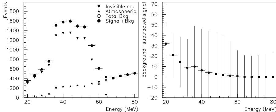
Figure 7: Supernova relic neutrino signal and backgrounds (left) and subtracted signal with statistical errors (right) in a 440 kt water cherenkov detector with a 10 years exposure. The selection efficiencies of SK were assumed; the efficiency change at 34 MeV is due to the spallation cut.
