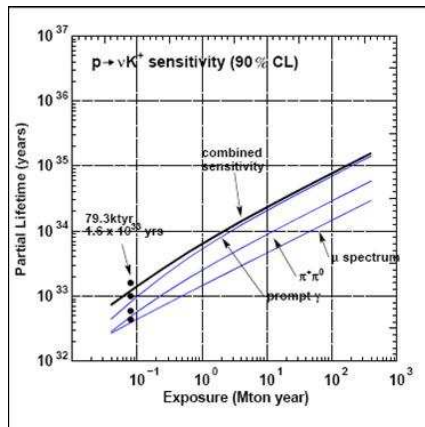
Figure 5: Expected sensitivity on \nu K^+ proton decay as a function of MEMPHYS exposure [4] (see text for details).
