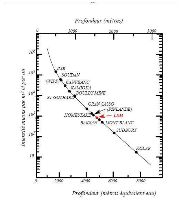
Figure 1: Muon flux as a function of overburden. The Frejus site is indicated by "LSM".
