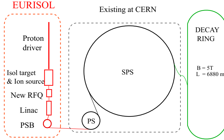
Figure 9: A schematic layout of the BetaBeam complex. On the left, the low energy part is largely similar to the EURISOL project [29]. The central part (PS and SPS) uses existing facilities. On the right, the decay ring has to be built.
