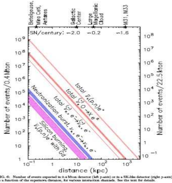
Figure 6: The number of events in a 400 kt water Čerenkov detector (left scale) and in SK (right scale) in all channels and in the individual detection channels as a function of distance for a supernova explosion [6].
