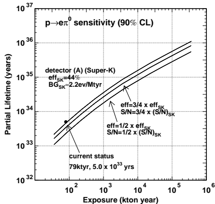
Figure 4: Sensitivity for e^+\pi^0 proton decay lifetime, as determined by UNO [4]. MEMPHYS corresponds to case (A).
