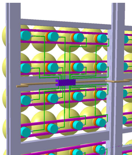
Figure 11: Sketch of a possible photo-sensor basic module composed of a matrix of 4 \times 4 12" PMTs with the electronic box containing the High Voltage unit and the Readout chip.
