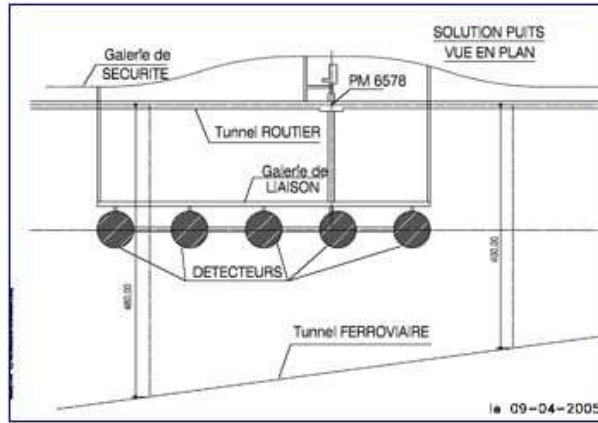
Figure 2: Envisaged configuration of the Fréjus underground laboratory.
