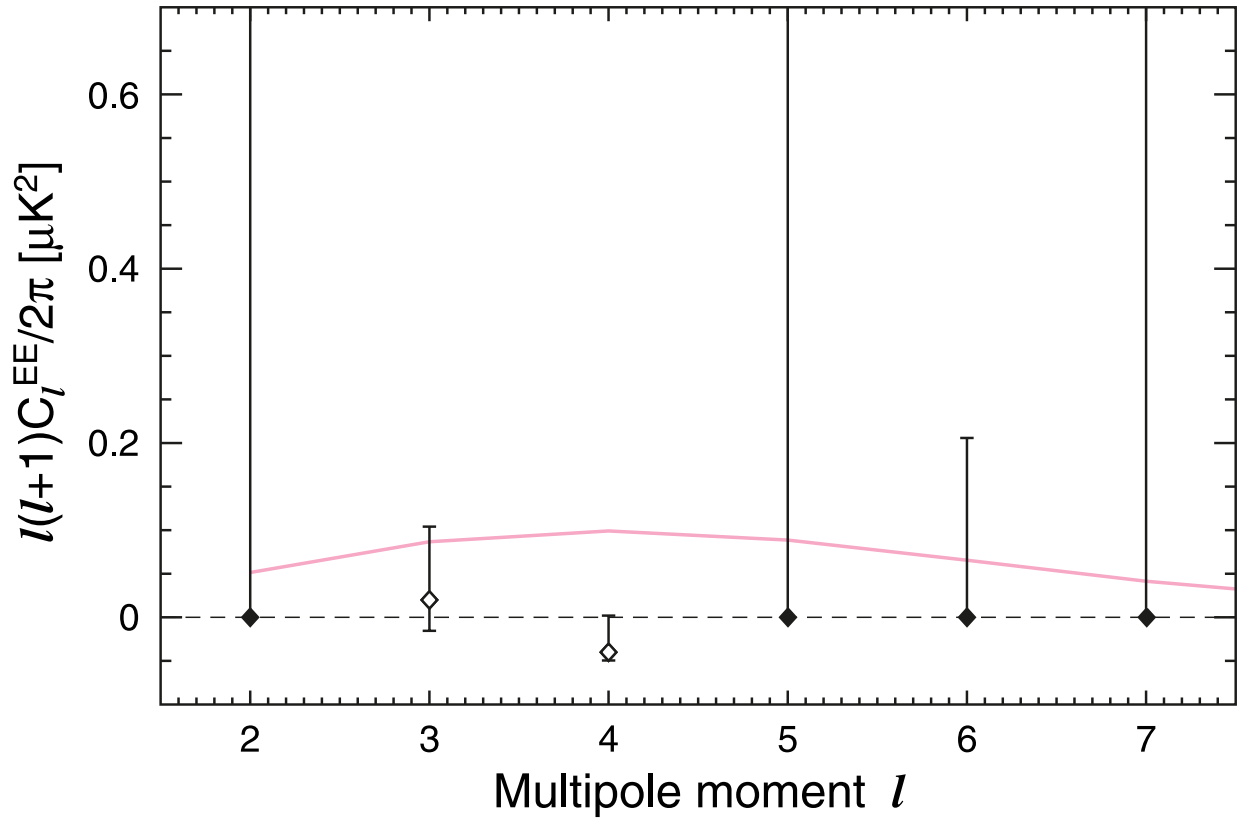
Fig. 10.— The EE power spectrum computed from the null sky maps, \frac{1}{2}S_{\text{Ka}} - \frac{1}{2}S_{\text{QV}} , where S = \text{Q,U} are the polarization Stokes parameters, and S_{\text{QV}} is the optimal combination of the Q and V band data. The pink curve is the best-fit theoretical spectrum from Dunkley et al. (2008). The spectrum derived from the null maps is consistent with zero.
