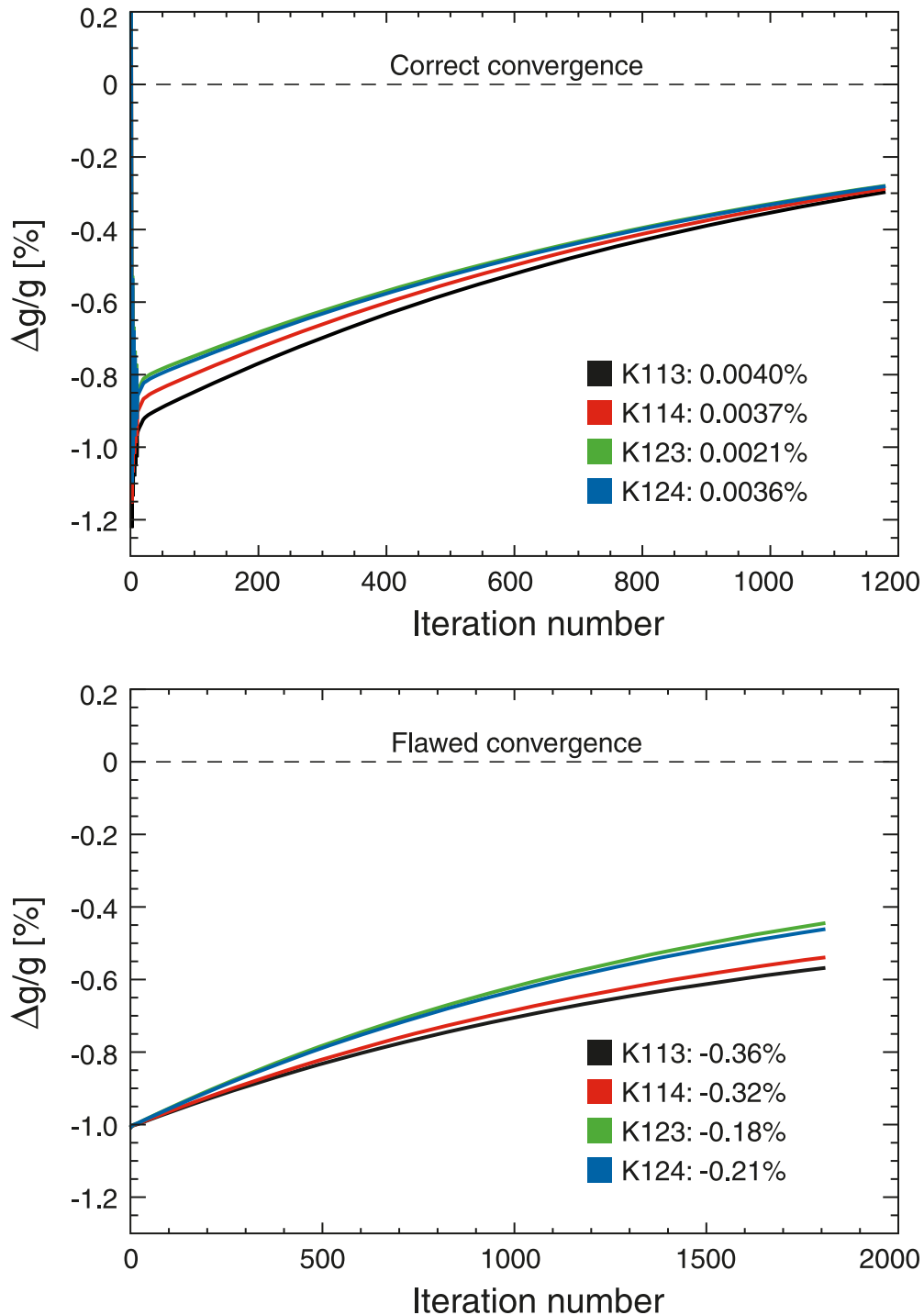
Fig. 6.— Gain convergence tests using the iterative sky map & calibration solver on a pair simulations. Both panels show the gain recovery as a function of iteration number for a 4-channel K band simulation. The initial guess was chosen to be in error by 1% to test convergence; the extrapolated output solutions are printed in each panel. top : Results for a noiseless simulation that includes a dipole signal (with Earth-velocity modulation) plus CMB and foreground anisotropy (the former is evaluated at the center frequency of each channel). The input gain was set to be constant in time. The extrapolated solutions agree with the input values to much better than 0.1%. bottom : Results for a noiseless simulation that includes only dipole signal (with Earth-velocity modulation) but no CMB or foreground signal. In this case the input gain was set up to have flight-like thermal variations. The extrapolated absolute gain recovery was in error by >0.3\% , indicating a small residual degeneracy between the sky model and the time-dependent calibration.
