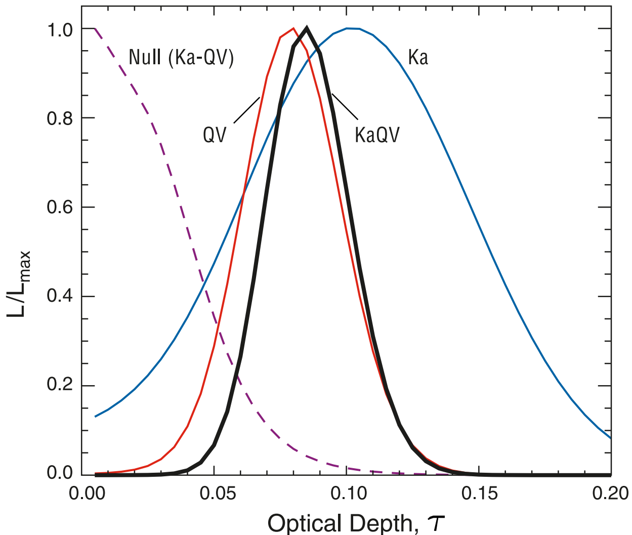
Fig. 11.— Estimates of the optical depth from a variety of data combinations. The dashed curve labeled Null uses the same null sky maps used in Figure 10. The optical depth obtained from Ka band data alone (blue) is consistent with independent estimates from the combined Q and V band data (red). The final 5 year analysis uses Ka, Q, and V band data combined (black). These estimates all use a 1-parameter likelihood estimation, holding other parameters fixed except for the fluctuation amplitude, which is adjusted to fit the first acoustic peak in the TT spectrum (Page et al. 2007). The degeneracy between \tau and other \Lambda CDM parameters is small: see Figure 7 of Dunkley et al. (2008).
