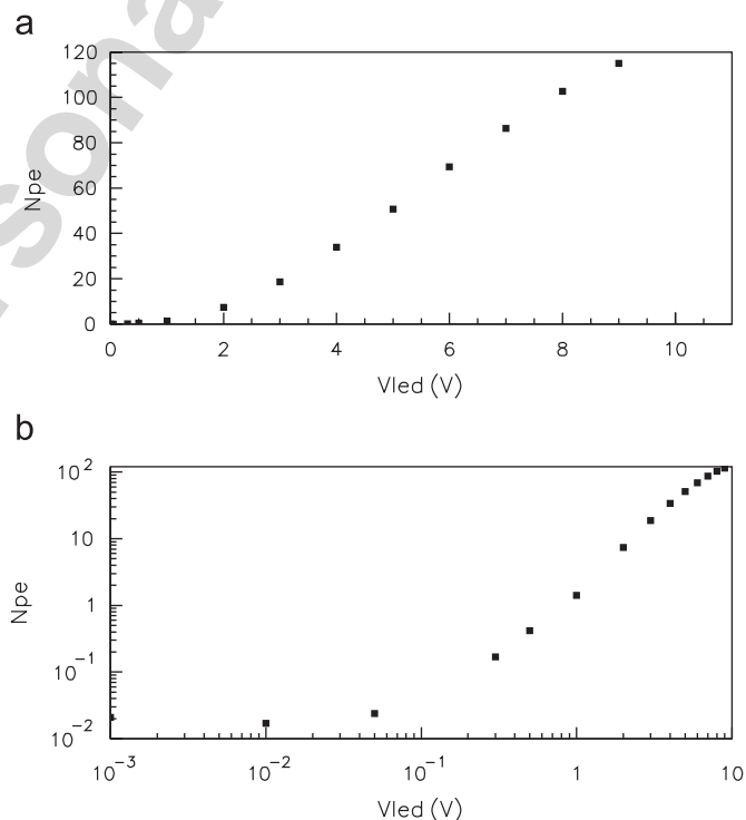
Fig. 27. Response of one channel as a function of the voltage applied to the LED: (a) linear scale showing the linearity at high voltage; (b) log/log scale showing the sensitivity at low voltage.
