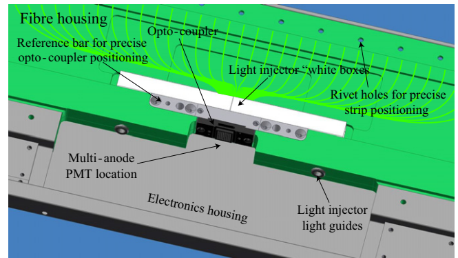
Fig. 12. Three-dimensional view of the central part of an end-cap.
