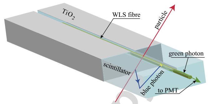
Fig. 1. Particle detection principle in a scintillating strip.
