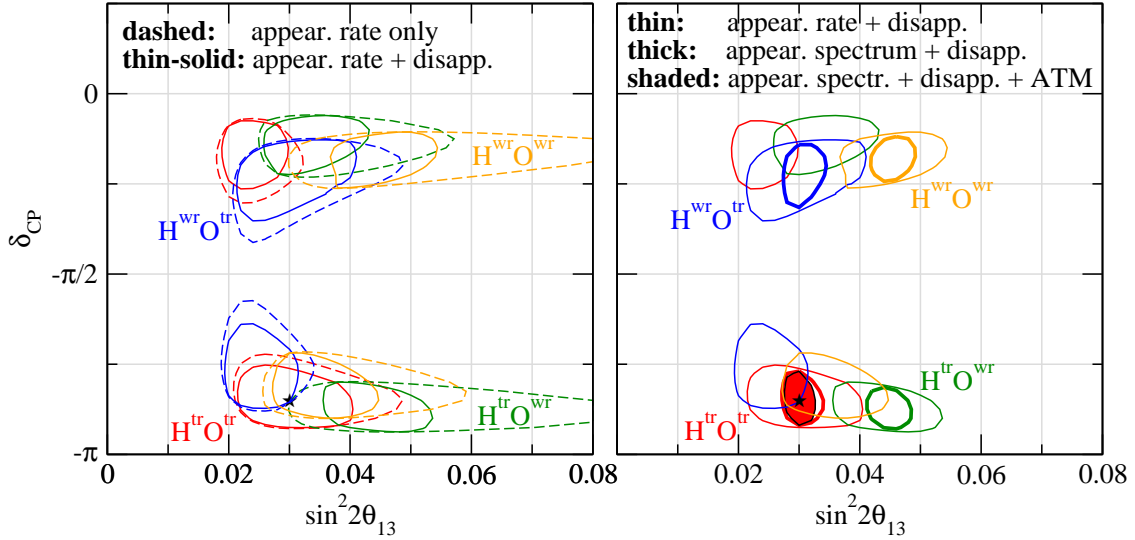
Figure 5: Resolving degeneracies in SPL by successively using the appearance rate measurement, disappearance channel, spectral information in the appearance channel, and atmospheric neutrinos. Allowed regions in \sin^2 2\theta_{13} and \delta_{\text{CP}} are shown at 95% CL, and \text{H}^{\text{tr/wr}}(\text{O}^{\text{tr/wr}}) refers to solutions with the true/wrong mass hierarchy (octant of \theta_{23} ). The true parameter values are \delta_{\text{CP}} = -0.85\pi , \sin^2 2\theta_{13} = 0.03 , \sin^2 \theta_{23} = 0.6 , and the values from Eq. (1) for the other parameters.
