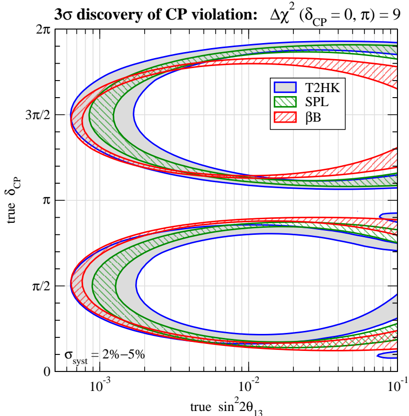
Figure 10: CPV discovery potential for \beta\text{B} , SPL, and T2HK: For parameter values inside the ellipse-shaped curves CP conserving values of \delta_{\text{CP}} can be excluded at 3\sigma ( \Delta\chi^2 > 9 ). The width of the bands corresponds to values for the systematical errors from 2% to 5%.
