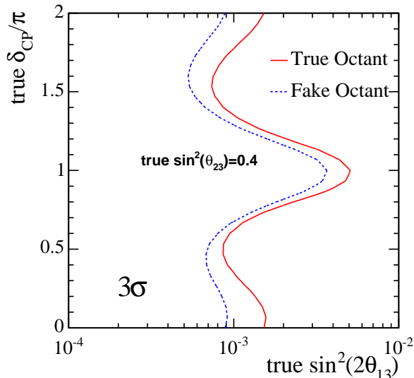
Figure 9: 3\sigma discovery sensitivity to \sin^2 2\theta_{13} for the SPL as a function of the true value of \delta_{\text{CP}} for \sin^2 \theta_{23}^{\text{true}} = 0.4 and true values for the other parameters as given in Eq. (1).
