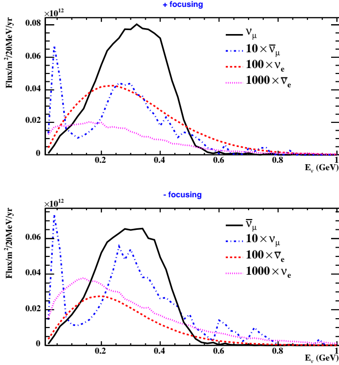
Figure 2: Neutrino fluxes, at 130 km from the target with the horns focusing the positive particles (top panel) or the negative particles (bottom panel). The fluxes are computed for a SPL proton beam of 3.5 GeV (4 MW), a decay tunnel with a length of 40 m and a radius of 2 m.
