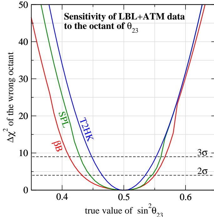
Figure 16: \Delta\chi^2 of the solution with the wrong octant of \theta_{23} as a function of the true value of \sin^2\theta_{23} . We have assumed a true value of \theta_{13} = 0 .
