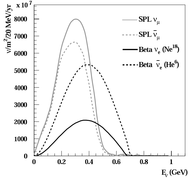
Figure 3: Comparison of the fluxes from SPL and \beta B .
