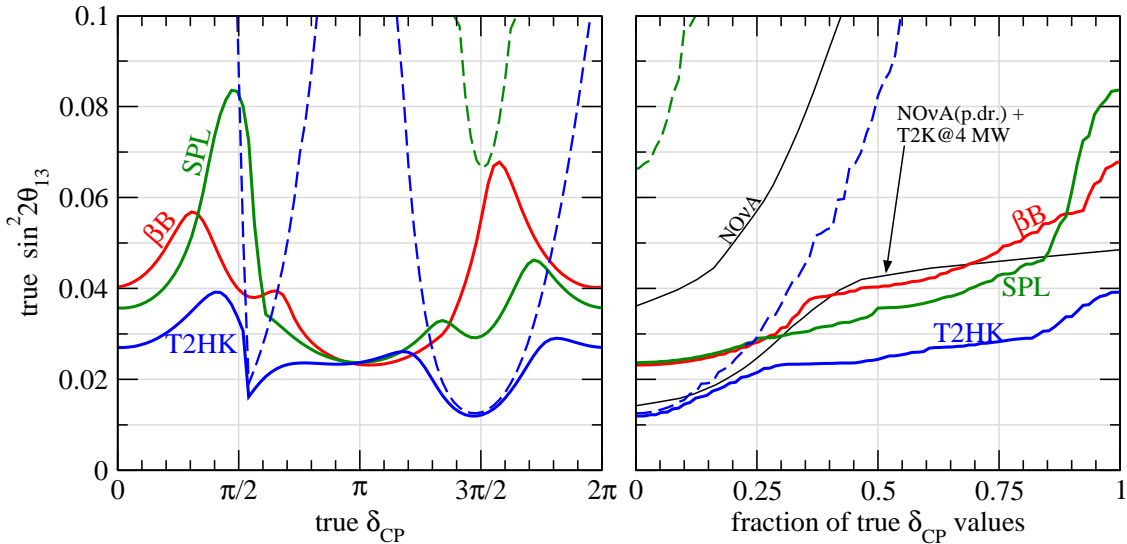
Figure 15: Sensitivity to the mass hierarchy at 2\sigma ( \Delta\chi^2 = 4 ) as a function of the true values of \sin^2 2\theta_{13} and \delta_{CP} (left), and the fraction of true values of \delta_{CP} (right). The solid curves are the sensitivities from the combination of long-baseline and atmospheric neutrino data, the dashed curves correspond to long-baseline data only. For comparison we show in the right panel also the sensitivities of NO \nu A and NO \nu A+T2K extracted from Fig. 13.14 of Ref. [16]. For the curve labeled “NO \nu A (p.dr.)+T2K@4 MW” a proton driver has been assumed for NO \nu A and the T2K beam has been up-graded to 4 MW, see Ref. [16] for details.
