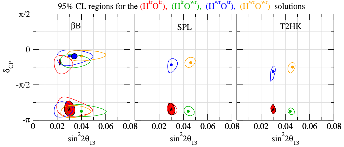
Figure 4: Allowed regions in \sin^2 2\theta_{13} and \delta_{\text{CP}} for LBL data alone (contour lines) and LBL+ATM data combined (colored regions). \text{H}^{\text{tr/wr}}(\text{O}^{\text{tr/wr}}) refers to solutions with the true/wrong mass hierarchy (octant of \theta_{23} ). The true parameter values are \delta_{\text{CP}} = -0.85\pi , \sin^2 2\theta_{13} = 0.03 , \sin^2 \theta_{23} = 0.6 , and the values from Eq. (1) for the other parameters.
