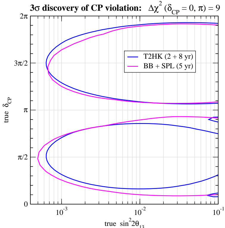
Figure 14: Sensitivity to CPV at 3\sigma ( \Delta\chi^2 > 9 ) for combining 5 yrs neutrino data from \beta B and SPL compared to 10 yrs data from T2HK (2 yrs neutrinos + 8 yrs antineutrinos).
