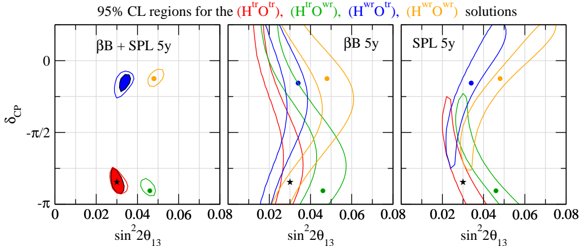
Figure 6: Allowed regions in \sin^2 2\theta_{13} and \delta_{\text{CP}} for 5 years data (neutrinos only) from \beta\text{B} , SPL, and the combination. \text{H}^{\text{tr/wr}}(\text{O}^{\text{tr/wr}}) refers to solutions with the true/wrong mass hierarchy (octant of \theta_{23} ). For the colored regions in the left panel also 5 years of atmospheric data are included; the solution with the wrong hierarchy has \Delta\chi^2 = 3.3 . The true parameter values are \delta_{\text{CP}} = -0.85\pi , \sin^2 2\theta_{13} = 0.03 , \sin^2 \theta_{23} = 0.6 , and the values from Eq. (1) for the other parameters. For the \beta\text{B} only analysis (middle panel) an external accuracy of 2% (3%) for |\Delta m_{31}^2| ( \theta_{23} ) has been assumed, whereas for the left and right panel the default value of 10% has been used.
