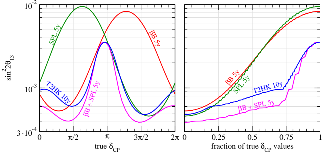
Figure 13: Discovery potential of a finite value of \sin^2 2\theta_{13} at 3\sigma ( \Delta\chi^2 > 9 ) for 5 yrs neutrino data from \beta B, SPL, and the combination of \beta B + SPL compared to 10 yrs data from T2HK (2 yrs neutrinos + 8 yrs antineutrinos).
