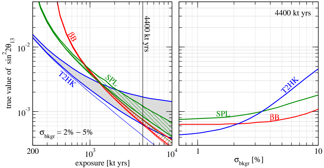
Figure 11: Impact of total exposure and systematical errors on the CPV discovery potential of \beta\text{B} , SPL, and T2HK. We show the smallest true value of \sin^2 2\theta_{13} for which \delta_{\text{CP}} = \pi/2 can be distinguished from \delta_{\text{CP}} = 0 or \delta_{\text{CP}} = \pi at 3\sigma ( \Delta\chi^2 > 9 ) as a function of the exposure in kt yrs (left) and as a function of the systematical error on the background \sigma_{\text{bkgr}} (right). The widths of the curves in the left panel corresponds to values of \sigma_{\text{bkgr}} from 2% to 5%. The thin solid curves in the left panel corresponds to no systematical errors. The right plot is calculated for the standard exposure of 4400 kt yrs. No systematical error on the signal has been assumed.
