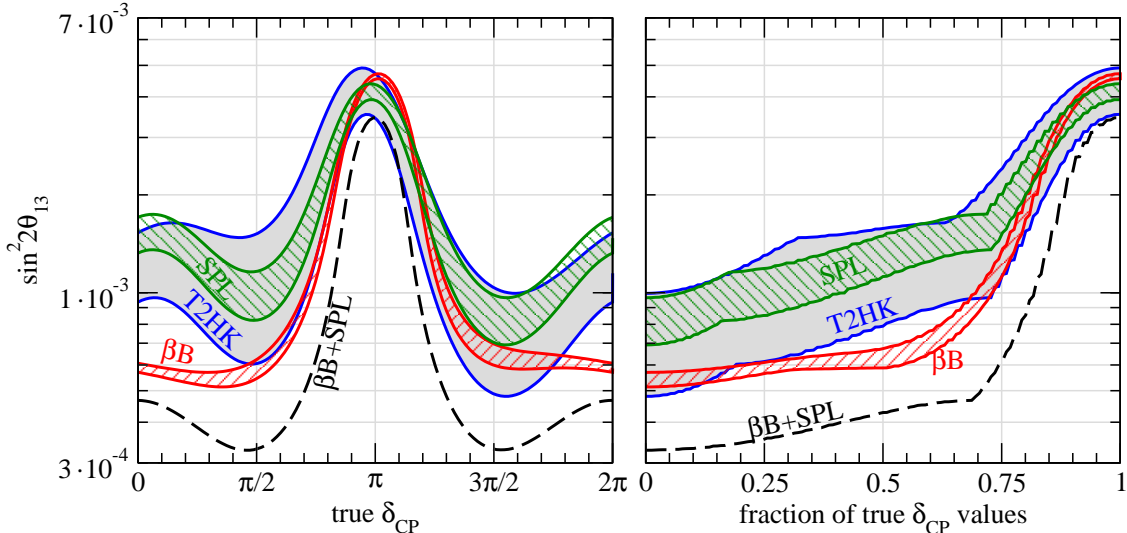
Figure 8: 3\sigma discovery sensitivity to \sin^2 2\theta_{13} for \beta B, SPL, and T2HK as a function of the true value of \delta_{\text{CP}} (left panel) and as a function of the fraction of all possible values of \delta_{\text{CP}} (right panel). The width of the bands corresponds to values for the systematical errors between 2% and 5%. The dashed curves correspond to the combination of \beta B and SPL with 10 yrs of total data taking each for a systematical error of 2%.
