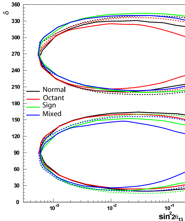
Figure 12: Impact of degeneracies on the CPV discovery potential for the \beta B. We show the sensitivity to CPV at 3\sigma ( \Delta\chi^2 > 9 ) computed for 4 different options about the true parameter values: Normal: \text{sign}(\Delta m_{31}^2) = 1 , \theta_{23} = 40^\circ ; Octant: \text{sign}(\Delta m_{31}^2) = 1 , \theta_{23} = 60^\circ ; Sign: \text{sign}(\Delta m_{31}^2) = -1 , \theta_{23} = 40^\circ ; Mixed: \text{sign}(\Delta m_{31}^2) = -1 , \theta_{23} = 60^\circ . Dotted curves are computed neglecting degeneracies.
