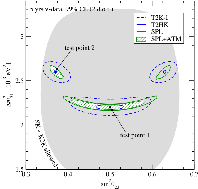
Figure 7: Allowed regions of \Delta m_{31}^2 and \sin^2 \theta_{23} at 99% CL (2 d.o.f.) after 5 yrs of neutrino data taking for SPL, T2K phase I, T2HK, and the combination of SPL with 5 yrs of atmospheric neutrino data in the MEMPHYS detector. For the true parameter values we use \Delta m_{31}^2 = 2.2(2.6) \times 10^{-3} \text{ eV}^2 and \sin^2 \theta_{23} = 0.5(0.37) for the test point 1 (2), and \theta_{13} = 0 and the solar parameters as given in Eq. (1). The shaded region corresponds to the 99% CL region from present SK and K2K data [11].
