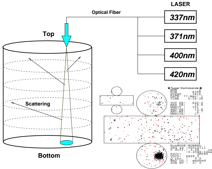
Fig. 31. Laser system for scattering and absorption parameter measurement, and a typical event.
