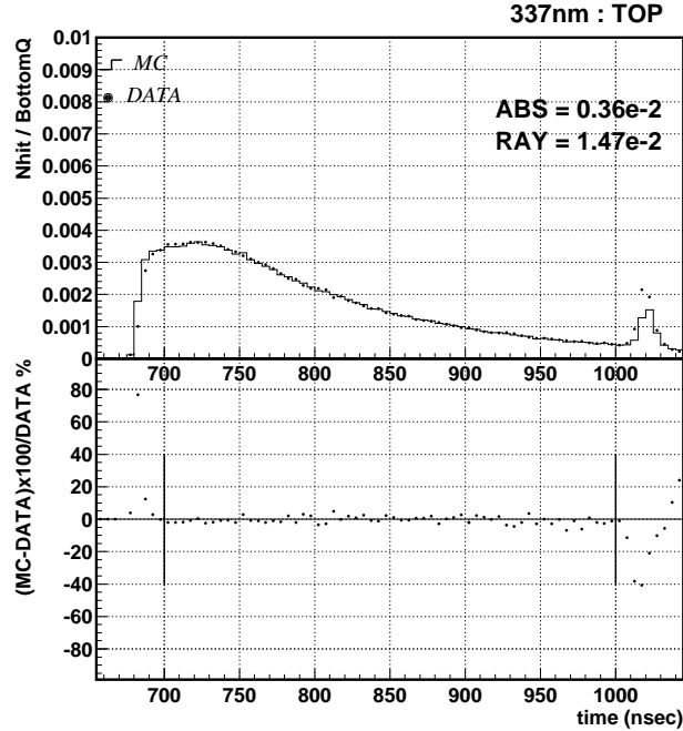
Fig. 32. The upper figure is the photon arrival-time distribution for the Monte Carlo (histogram) and data (dots). The lower figure is the ratio between MC and data as a function of time.
