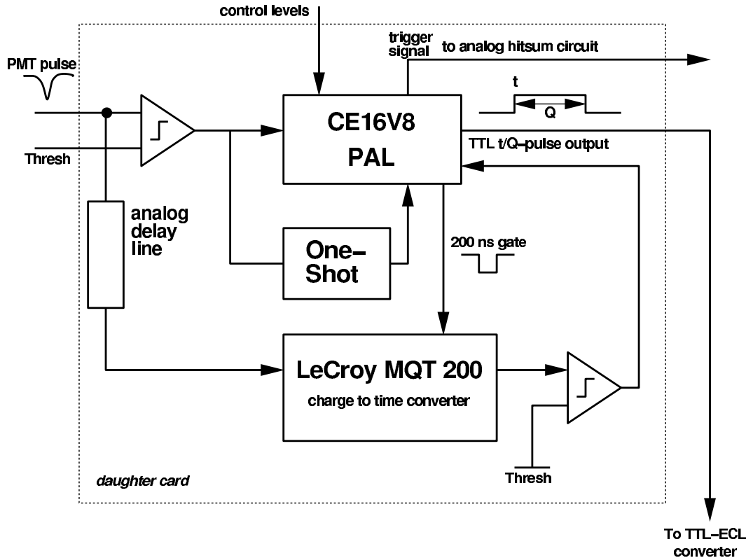
Fig. 19. Block diagram for a single QTC module.
