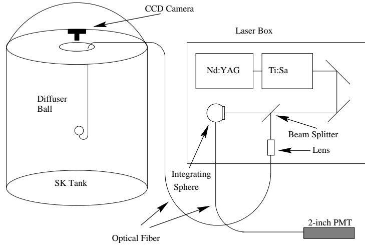
Fig. 25. Laser system for water attenuation length measurement.
