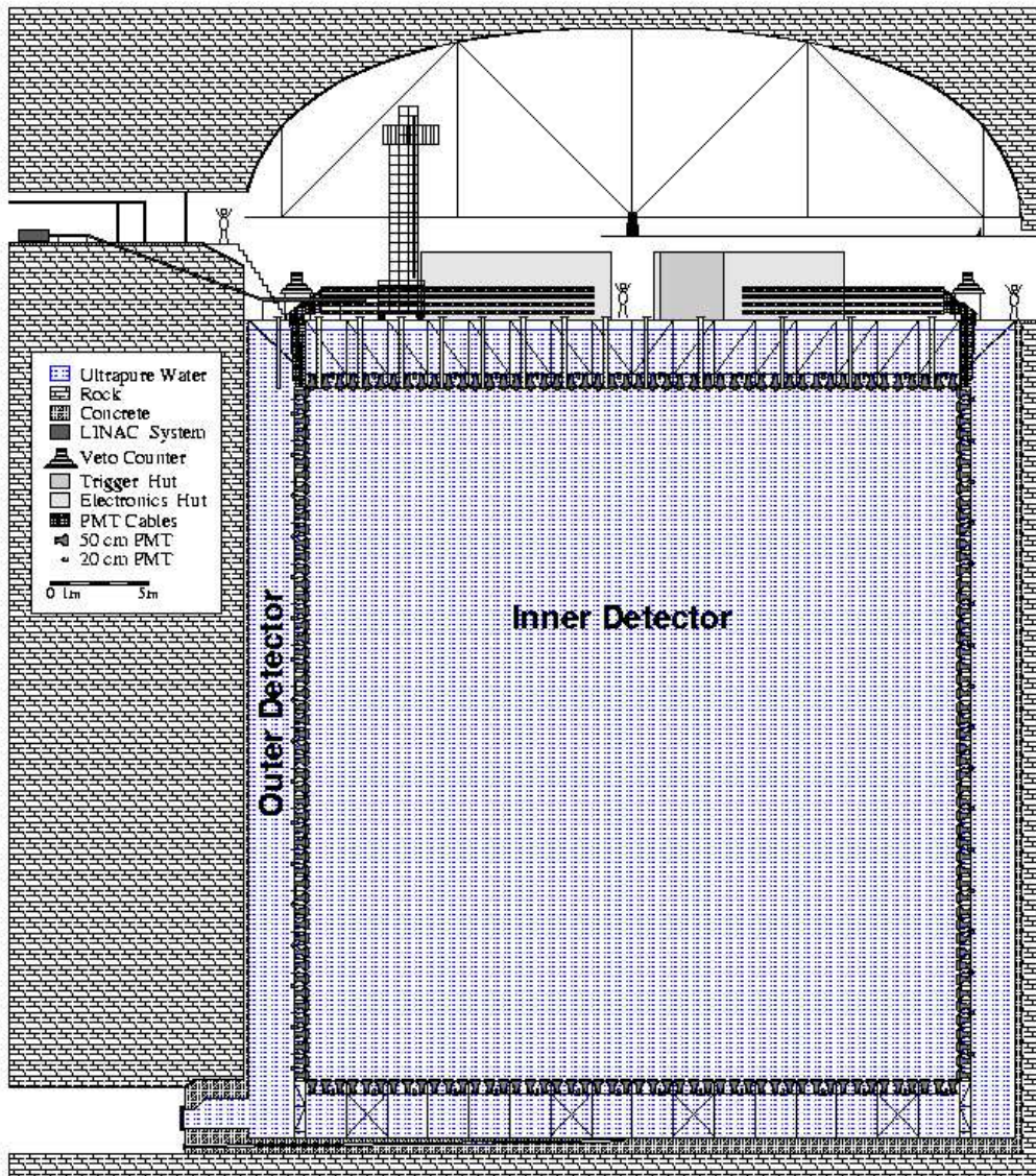
Fig. 6. A cross section of the Super-Kamiokande detector
