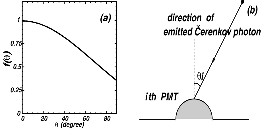
Fig. 28. Relative photo-sensitivity: (a) Measurement result, (b) Definition of the incident angle
