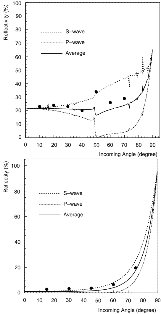
Fig. 12. Reflectivity of PMT surface(top panel) and the opaque sheets used to fill gaps between PMTs (bottom panel). Points show the results of measurements, and lines show calculated values: the dashed line shows the S-wave, the dotted line shows P-wave and the solid line shows the averaged value.
