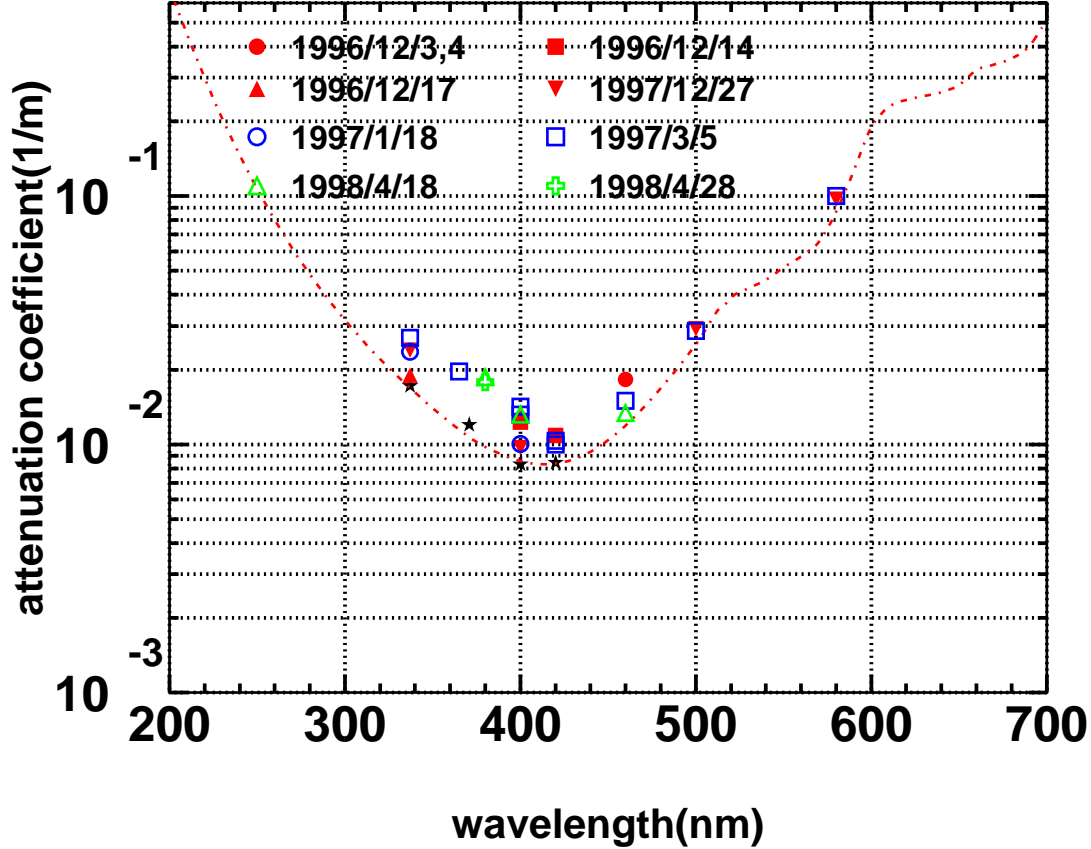
Fig. 27. Water attenuation length.
