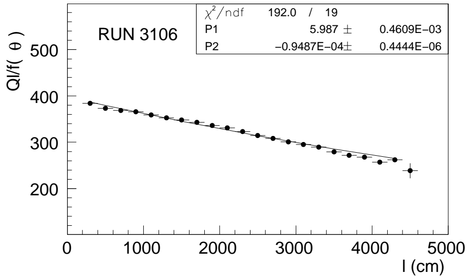
Fig. 29. Effective observed charge as a function of the path length.
