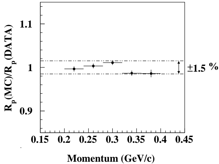
Fig. 48. Comparison of the ratio R , the measured to inferred momentum from the Cherenkov angle with the Monte Carlo prediction. The double ratio R(MC)/R(data) is plotted.
