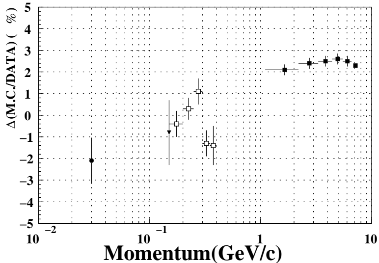
Fig. 51. Comparison of momentum measurements in the range 30 MeV/c to 10 GeV/c. Solid squares represent measurements with high energy stopping muons; open squares, low energy stopping muons; solid triangles, single \pi^0 s; solid circles, decay electrons.
