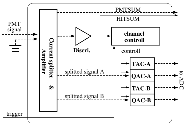
Fig. 13. A schematic view of the analog input block of the ATM. Only one channel is shown in the figure. Dashed arrows show the PMT signal, its split signals, and accumulated TAC/QAC signals. Solid arrows show the logic signals which control the processing of the analog signals.
