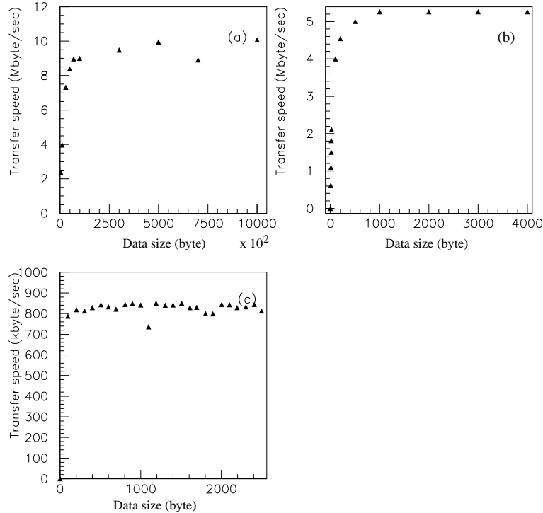
Fig. 16. Measured data transfer speed for (a) SMP \rightarrow on-line server, (b) Sparse Data Scan and (c) TRG \rightarrow on-line server as a function of data size.
