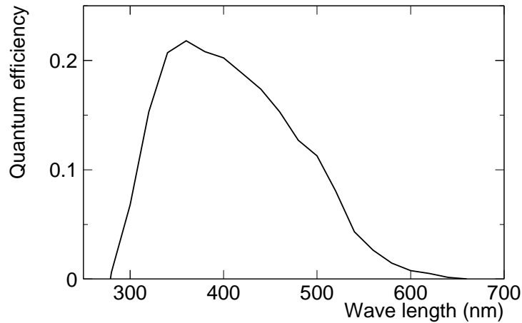
Fig. 8. Quantum efficiency of the photocathode as a function of wavelength.
