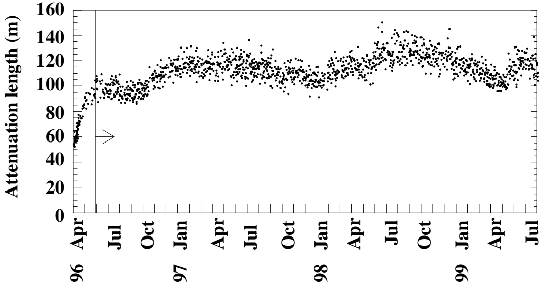
Fig. 30. Time variation of the water attenuation length.
