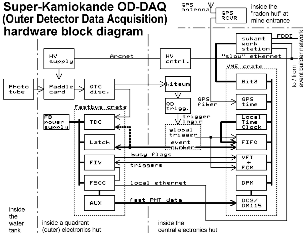
Fig. 18. OD DAQ block diagram and data flow.
