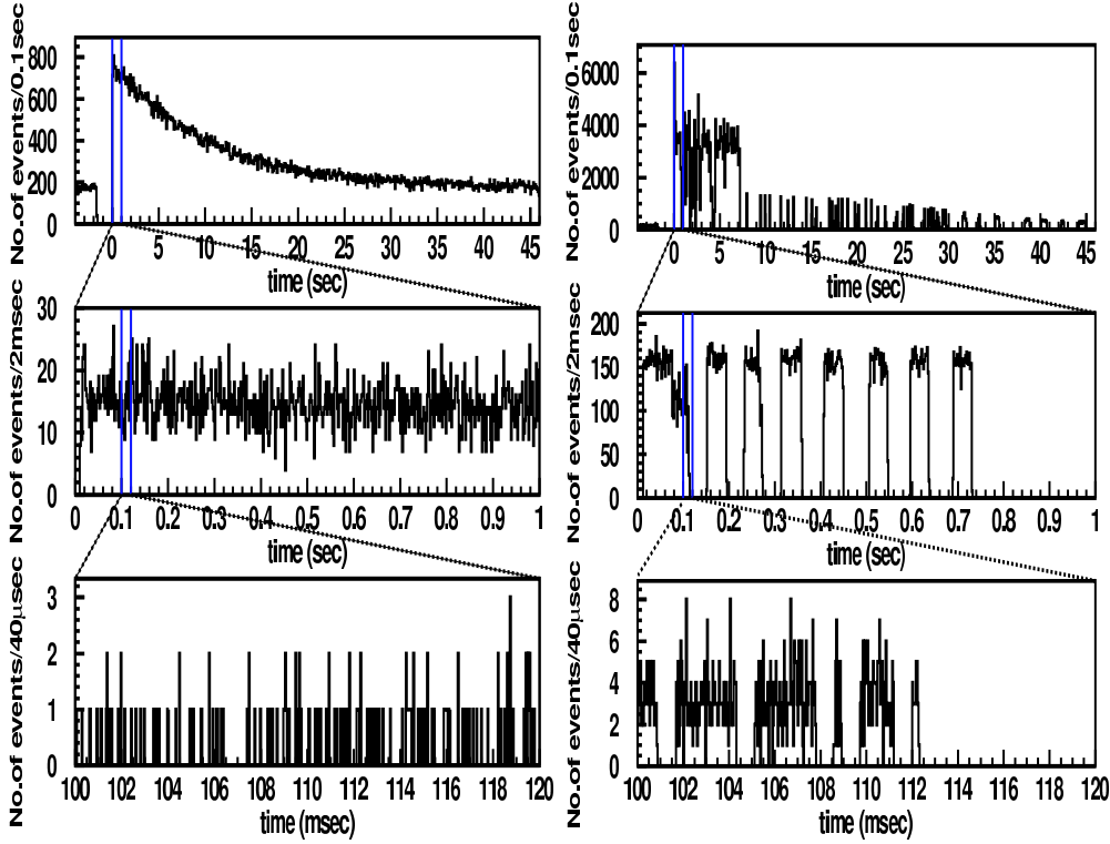
Fig. 17. Event rate variation as a function of time after beginning of a trigger burst, for 7.5 kHz burst (left), and 75 kHz burst (right). Bin sizes are (top) 0.1 s, (middle) 2 ms, and (bottom) 40 \mu s, respectively. No deadtime is observed for bursts up to 12 kHz. However, there are blank areas due to deadtime in the right-hand figure (middle and bottom) after 0.1 s.
