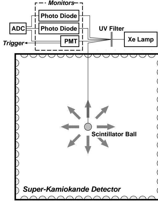
Fig. 34. The relative gain measurement system.
