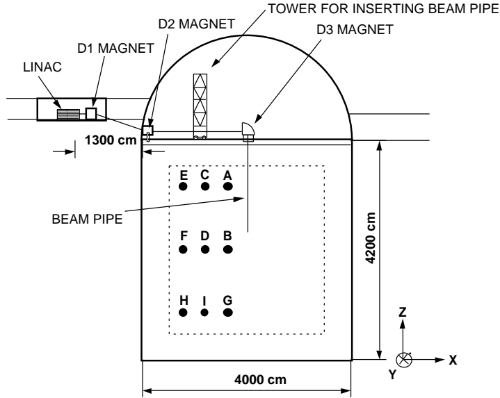
Fig. 40. LINAC system. The lettered positions indicate the locations where the end of the beam pipe is positioned in the tank for LINAC data taking.
