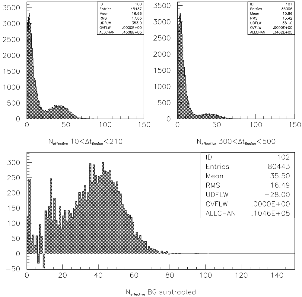
Fig. 45. N_{eff} distributions: (a) Top left. Distribution with 10 \leq \Delta t \leq 210 \mu s , (b) Top right. Distribution with 300 \leq \Delta t \leq 500 \mu s , (c) Bottom. Distribution after background subtraction.
