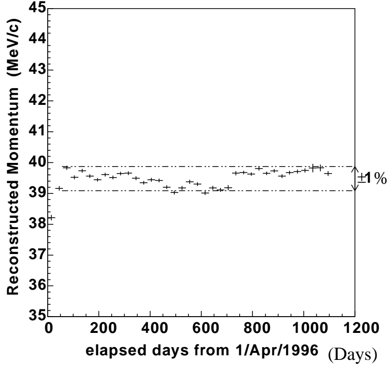
Fig. 47. The mean energy of decay electrons as a function of time.
