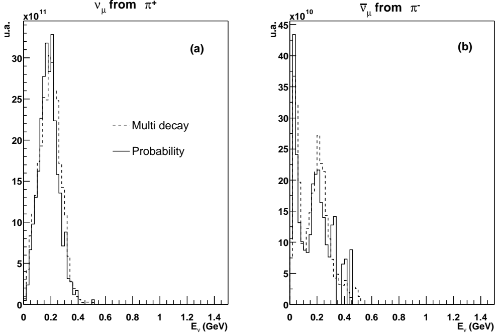
Fig. 6. Comparison between the probability method, (—) curve, and the full GEANT simulation method, (- - -) curve, for the \nu_\mu from \pi^+ flux (a) and the \bar{\nu}_\mu from \pi^- flux (b). The horns are set to focus positive particles. It should be stressed that the full GEANT simulation has taken roughly 13 times more CPU time than the probability method with the same number of protons on target, and the later simulation is able to produce as well the \nu_e and \bar{\nu}_e fluxes contrary to the former simulation.
