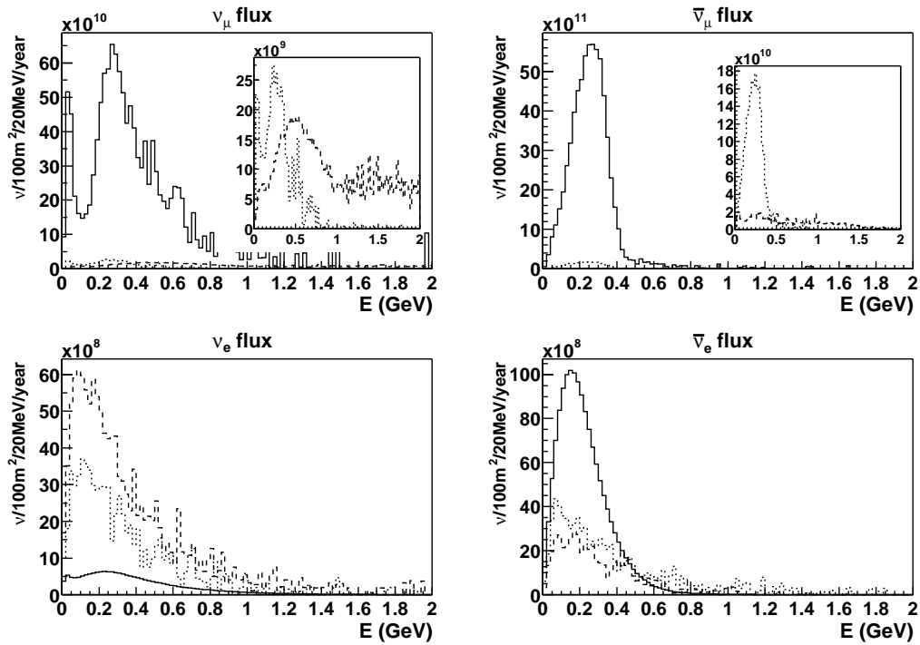
Fig. 12. Same legend as for figure 8 but for proton beam kinetic energy of 8 GeV (4 MW).
