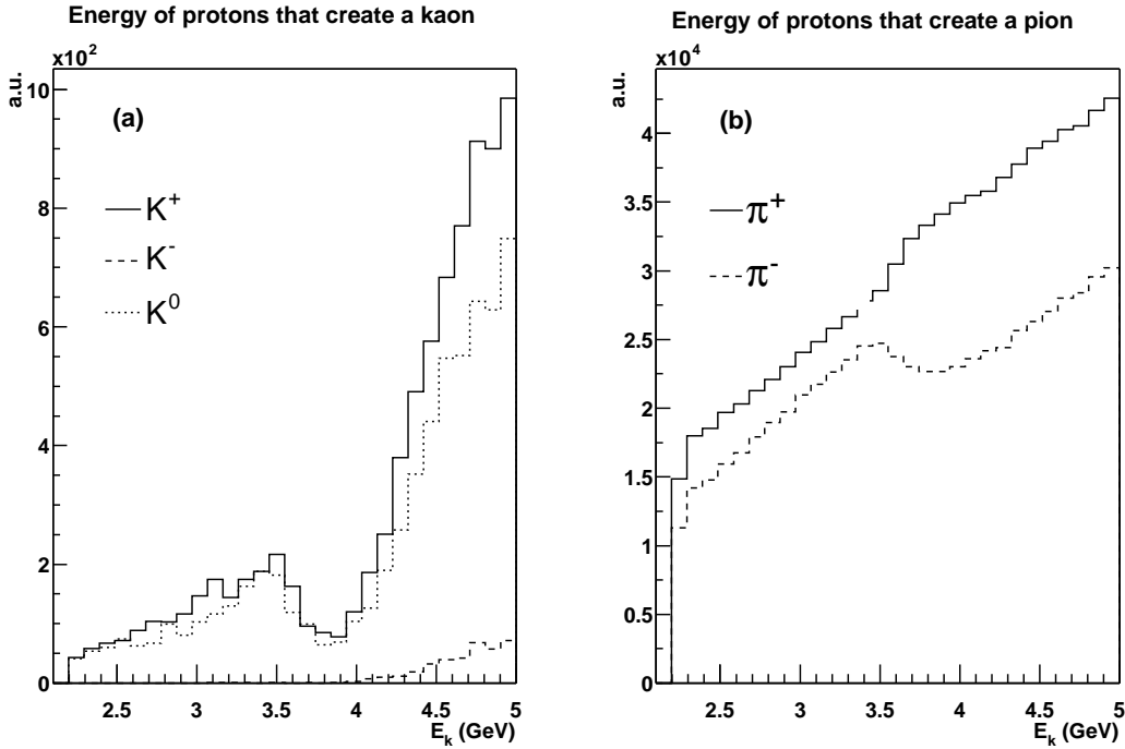
Fig. 4. Kaon production (a) as a function of the incident proton beam kinetic energy ( E_k ) for 10^6 incident protons with (—) curve for K^+ , (- - -) curve for K^- and (· · · · ·) curve for K^0 . Pion production (b) in the same conditions with (—) curve for \pi^+ and (- - -) curve for \pi^- .
