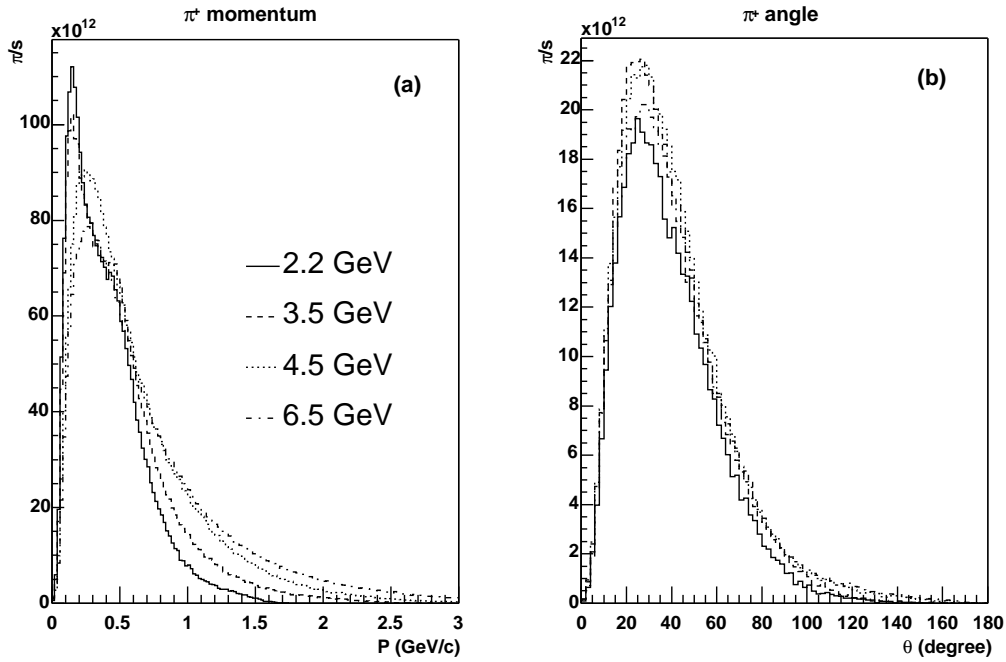
Fig. 2. (a) \pi^+ momentum distribution per second at the exit of the target for the different proton beam energies studied, simulated with FLUKA, and (b) \pi^+ angle with respect to the beam axis of the pion having a momentum between 0.5 GeV/c and 0.7 GeV/c. The different SPL beam kinetic energies presented are (—) 2.2 GeV, (- - -) 3.5 GeV, (· · · · ·) 4.5 GeV and (— · —) 6.5 GeV.
