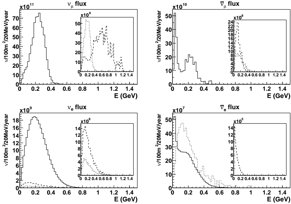
Fig. 7. Neutrino fluxes, 100 km from the target and with the horns focusing the positive particles. The fluxes are computed for a SPL proton beam of 2.2 GeV (4 MW), a decay tunnel with a length of 20 m and a radius of 1 m. The top left panel contains the \nu_\mu fluxes, and the top right panel shows the \bar{\nu}_\mu fluxes. The bottom left panel presents the \nu_e fluxes while the bottom right panel displays the \bar{\nu}_e fluxes. The (—) curve is the contribution from primary pions and the daughter muons, and from primary muons. The (- - -) curve is the contribution from the charged kaon decay chain, and the (· · · · ·) curve is the contribution from the K^0 decay chain. An insert has been added to the plots to highlight when needed the contribution of charged and neutral kaons.
