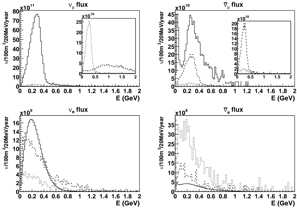
Fig. 11. Same legend as for figure 7 but for proton beam kinetic energy of 8 GeV (4 MW).
