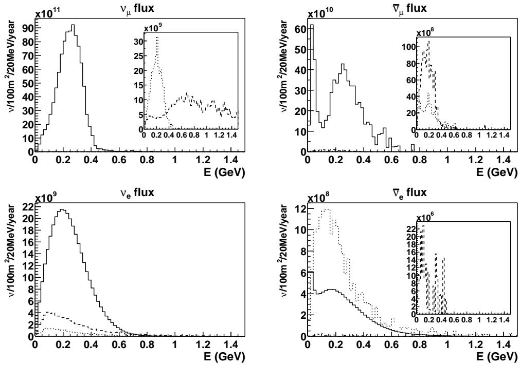
Fig. 9. Same legend as for figure 7 but for proton beam kinetic energy of 3.5 GeV (4 MW).
