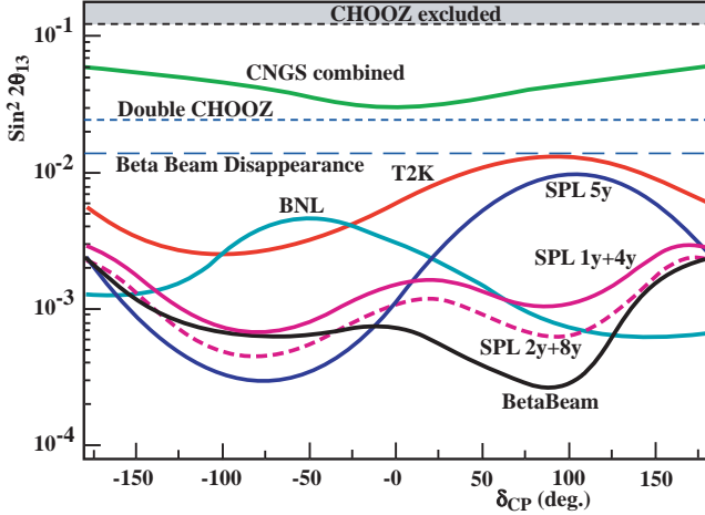
Fig. 18. 90%CL sensitivity contours labeled by the project or experiment involved. The "CHOOZ excluded" dashed curve comes from the exclusion obtained from reference [10] with \Delta m^2 = \Delta m_{atm}^2 ; in the same conditions is given the sensitivity foreseen for the "Double-CHOOZ" project [11]. The "CNGS combined" has been obtained combining the results from OPERA and ICARUS [41]. The T2K contour has been derived from reference [42]. The BNL contour has been obtained from reference [43]. The "Beta Beam" contour has been computed with 5 years running with both \nu_e and \bar{\nu}_e neutrino beams in an appearance mode, while the dashed "Beta Beam disappearance" has been obtained as if the \beta beam were analysed like a reactor experiment with 1% systematic error [44]. The "SPL 5y" and "SPL 2y+8y" and "SPL 1y+4y" curves have been obtained from the optimisation described in this paper ("5y": positive only focusing scenario; "1y+4y": 1 year of positive focusing and 4 years of negative focusing scenario; "2y+8y": 2 years of positive focusing and 8 years of negative focusing scenario) using a 3.5 GeV beam and a decay tunnel of 40 m length, and 2 m radius.
