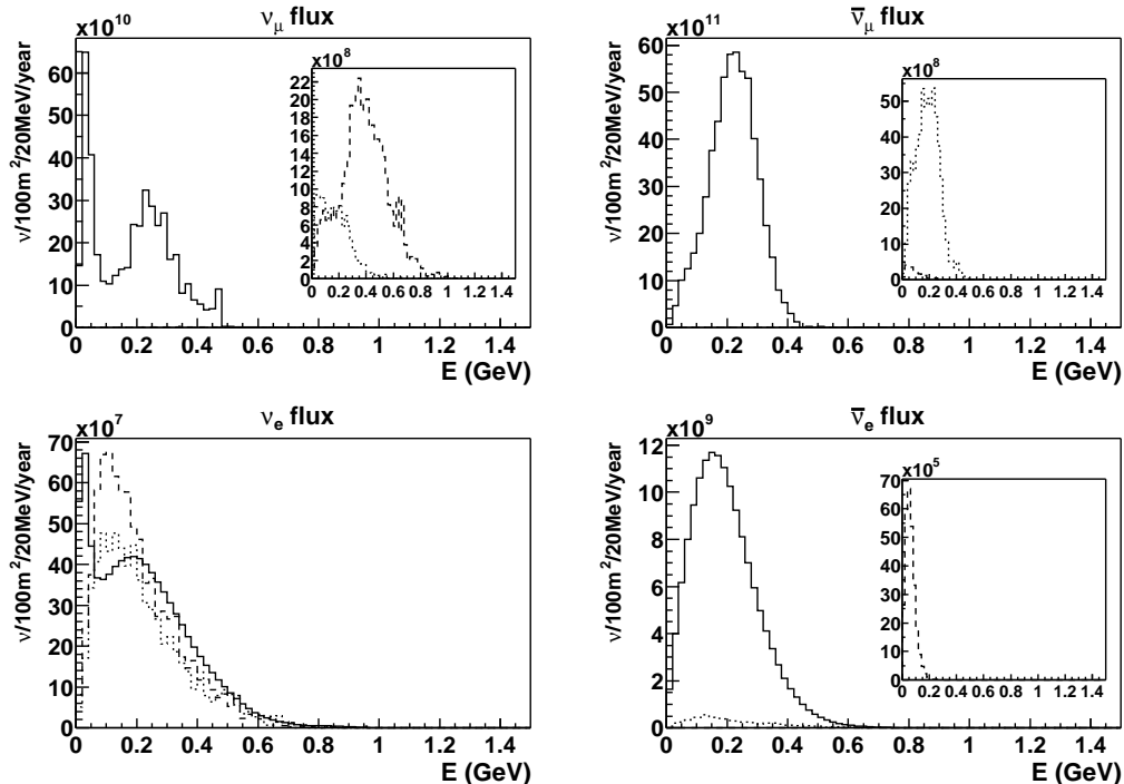
Fig. 8. Same legend as for figure 7 but the horns are focusing negative particles.
