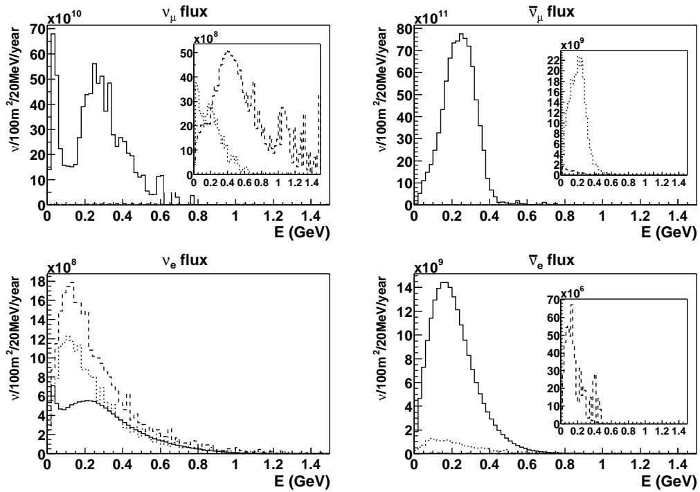
Fig. 10. Same legend as for figure 8 but for proton beam kinetic energy of 3.5 GeV (4 MW).
