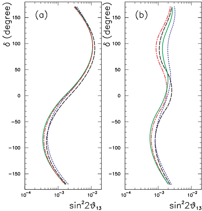
Fig. 16. 90% sensitivity contours obtained with SPL beam energy of 2.2 GeV (---), 3.5 GeV (— · —), 4.5 GeV (—) and 8 GeV (·····) at 90% CL. Default parameters of table 6 are used either with a 5 years positive focusing scenario (a) or a mixed scenario of 2 years positive focusing and 8 years of negative focusing (b). In particular, it is reminded that the tunnel geometry parameters are L_T = 20 m and R_T = 1 m.
