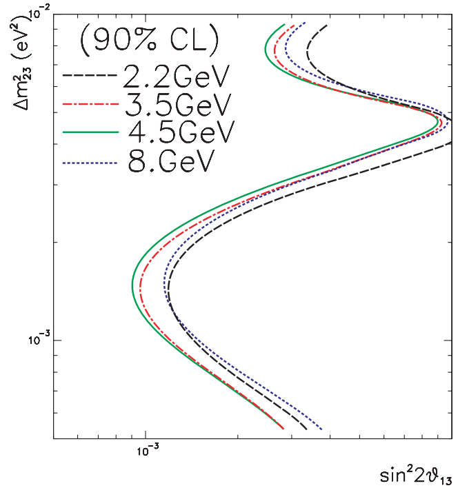
Fig. 14. Comparison of 90% CL sensitivity contours obtained with SPL energies of 2.2 GeV (---), 3.5 GeV (— · —), 4.5 GeV (—) and 8 GeV (·····) and default parameters of table 6. In particular, it is reminded that the tunnel geometry parameters are L_T = 20 m and R_T = 1 m.
