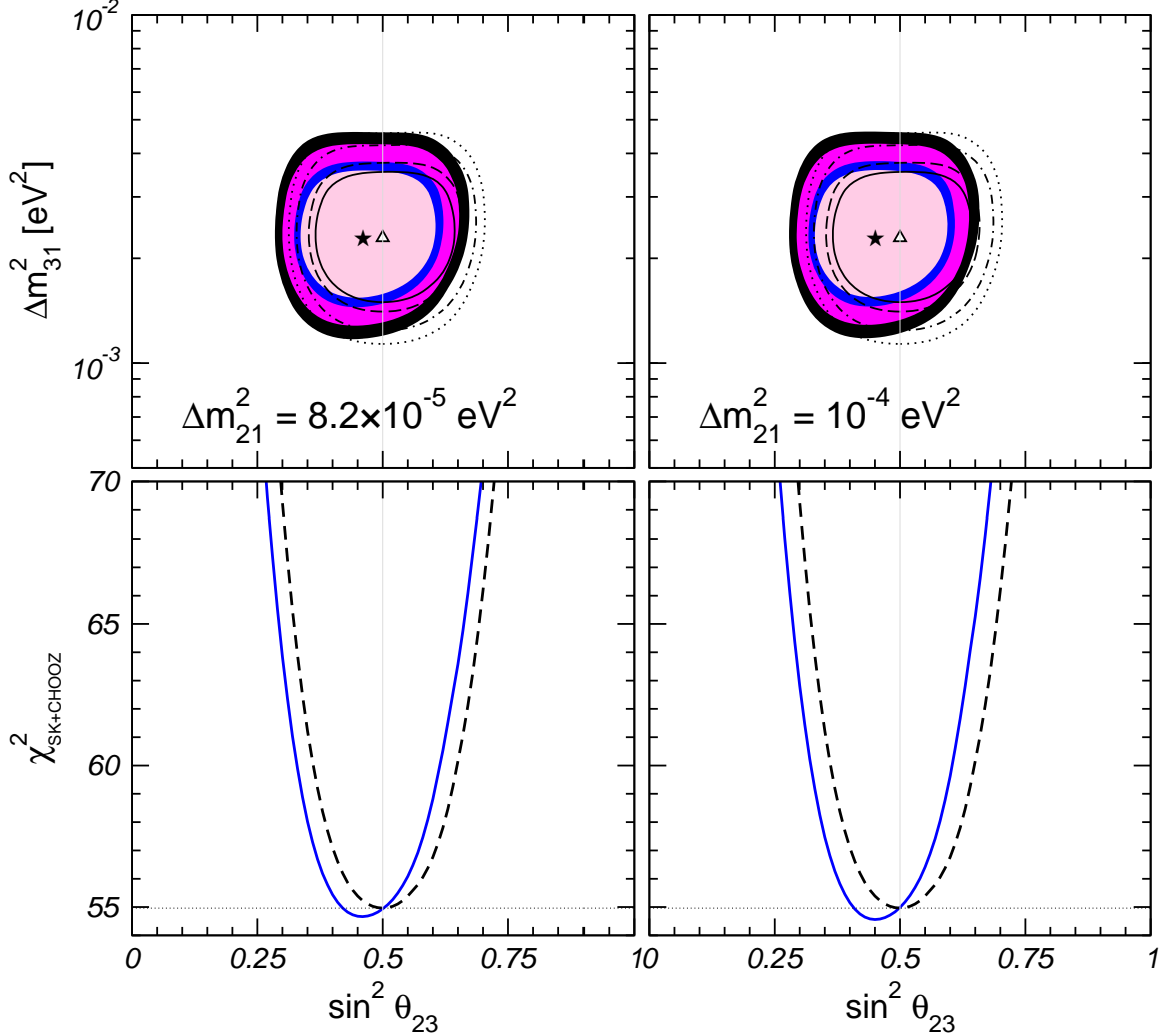
FIG. 2: Allowed regions (90%, 95%, 99% and 3\sigma C.L.) of the oscillation parameters \Delta m^2_{31} and \sin^2 \theta_{23} from the combined analysis of all the atmospheric and CHOOZ data samples. The best fit points are marked with either a star or a triangle. In the lower panels we show the dependence of the \chi^2 function on \theta_{23} , marginalized with respect to \Delta m^2_{31} . Colored regions, stars and solid blue lines correspond to \tan^2 \theta_{12} = 0.42 , \theta_{13} free and \Delta m^2_{21} set to the value indicated in each panel. Hollow regions, triangles and dashed black lines are for \Delta m^2_{21} = 0 and \theta_{13} free.
