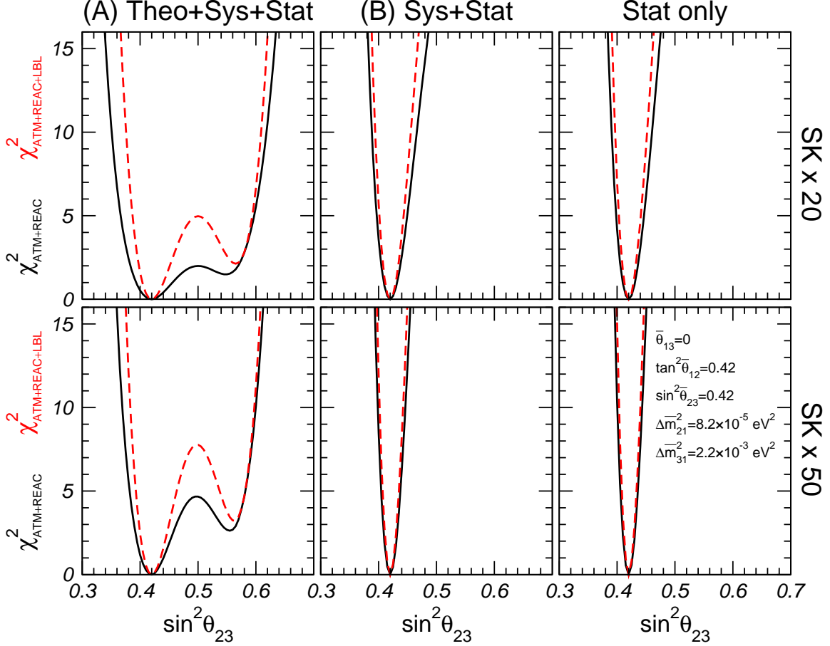
FIG. 5: Dependence of \chi^2_{\text{ATM+REAC}} (full black line) and \chi^2_{\text{ATM+REAC+LBL}} (red dashed line) on \sin^2 \theta_{23} , for \Delta m_{31}^2 = 2.2 \times 10^{-3} \text{ eV}^2 and setting the simulated point ( \bar{\omega} ) to \bar{\theta}_{13} = 0 , \tan^2 \bar{\theta}_{12} = 0.42 , \Delta \bar{m}_{21}^2 = 8.2 \times 10^{-5} \text{ eV}^2 , \sin^2 \bar{\theta}_{23} = 0.42 and \Delta \bar{m}_{31}^2 = 2.2 \times 10^{-3} \text{ eV}^2 . For the definition of \chi^2_{\text{ATM+REAC}} and \chi^2_{\text{ATM+REAC+LBL}} see Eqs. (20) and (22).
