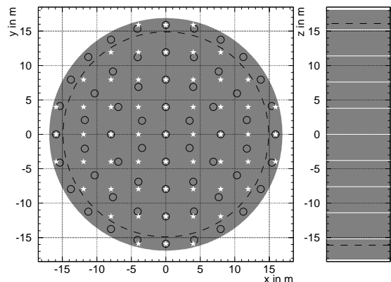
FIG. 7: Search grid for the vertex reconstruction in the xy plane and in z . The shaded area is the SK inner detector volume. The dashed line indicates the fiducial volume. The white stars (white lines) are the grid points used by the standard vertex reconstruction. The black circles are used by the second vertex reconstruction.
