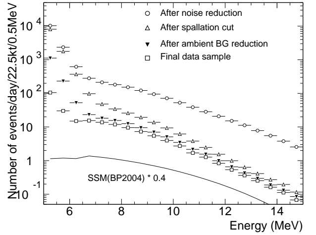
FIG. 39: Summary of the data reduction steps.
