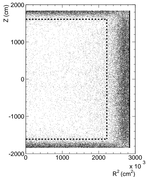
FIG. 25: Typical vertex distribution of the low energy events before the Intelligent Trigger selection. The analysis energy threshold for this plot is 5.0 MeV. The dashed line shows the fiducial volume edge.
