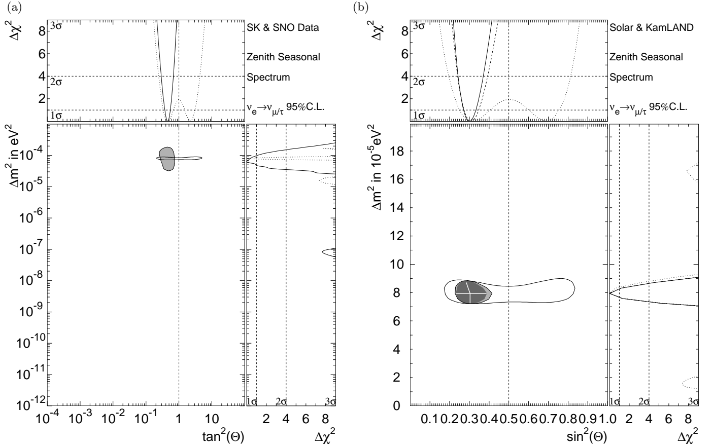
FIG. 56: (a) Allowed area at 95% C.L. from the combination of SK and SNO. The graphs at the top (and right) show the \chi^2 difference as a function of \tan^2 \theta ( \Delta m^2 ) only: the solid line is the SK/SNO fit, the dotted line results from KamLAND [18] data. The lines inside the contours show which \Delta m^2 ( \tan^2 \theta ) is chosen. (b) Allowed area at 95% C.L. from the combination of SK/SNO (gray) and all solar data (dark gray), and from the combination of solar and KamLAND data (light gray). Note the linear scale of both axes. Only LMA-I remains allowed. Overlaid is the region allowed by KamLAND alone.
