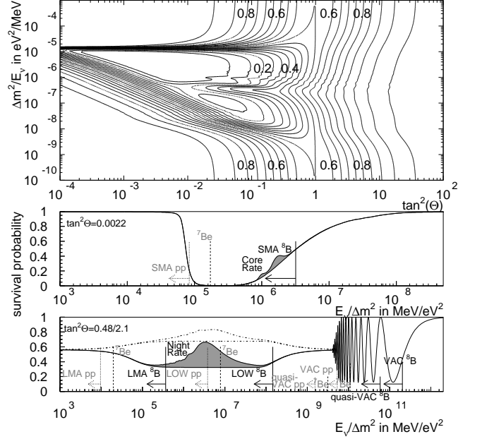
FIG. 48: Survival probability for {}^8\text{B} solar neutrinos. The top plot displays contours of equal probability as a function of \Delta m^2/E and \tan^2 \theta . The middle panel shows the same probability as a function of E/\Delta m^2 only where a particular (small) mixing angle has been selected. The shaded area contrasts the difference between neutrinos passing through the core of the Earth (which has the highest matter density) with neutrinos arriving directly from the Sun. The bottom panel shows a large mixing case. The line above the shaded area depicts the average probability for neutrinos passing through the Earth. Superimposed on these two lower panels are the locations of three neutrino branches ( pp – dotted, {}^7\text{Be} – dashed, and {}^8\text{B} – solid) for the SMA, LMA, LOW, VAC, and quasi-VAC solutions.
