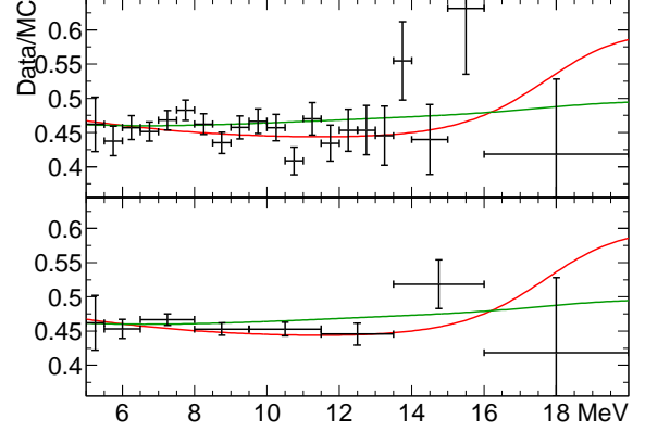
FIG. 51: Distortion of the recoil electron spectrum using 21 (upper panel) and 8 (lower panel) bins. The measured event rates in each bin are divided by the event rates expected from MC assuming a {}^8\text{B} \nu flux of 5.076 \times 10^6 / \text{cm}^2\text{s} and a hep \nu flux of 32 \times 10^6 / \text{cm}^2\text{s} . Overlaid is a typical LMA solution (red) and a LOW solution (green), where the assumed neutrino fluxes were fit to best describe the data.
