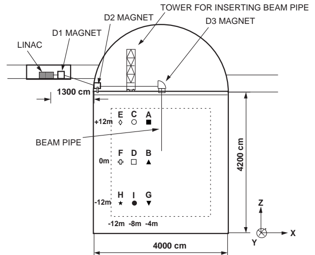
FIG. 18: The LINAC system at SK. The dotted line represents the fiducial volume of the detector and the black dots indicate the positions where LINAC data were taken.
