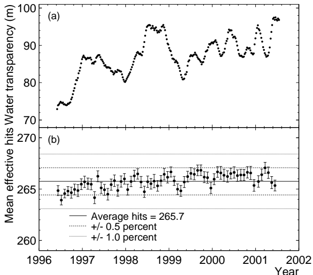
FIG. 17: (a) Time variation of the measured water transparency during SK-I. Stability of the SK-I energy scale as a function of time. (b) Each point represents the mean N_{eff} value for 28 days of \mu -e data. The solid line represents the average N_{eff} for all \mu -e events in SK-I; the dashed and dotted lined represent, respectively, \pm 0.5\% and \pm 1.0\% deviations from the average.
