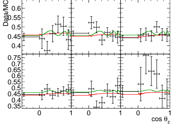
FIG. 52: Dependence of Data/MC on solar zenith angle. The MC assumes a {}^8\text{B} \nu flux of 5.076 \times 10^6 / \text{cm}^2\text{s} and a hep \nu flux of 32 \times 10^6 / \text{cm}^2\text{s} . The six panels correspond to the energy ranges 5.5-6.5 MeV, 6.5-8.0 MeV, 8.0-9.5 MeV, 9.5-11.5 MeV, 11.5-13.5 MeV, and 13.5-16.0 MeV. Overlaid is a typical LMA solution (red) and a LOW solution (green), where the assumed neutrino fluxes were fit to best describe the data.
