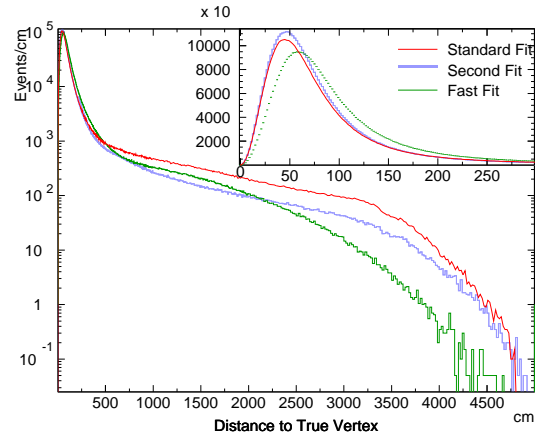
FIG. 10: Distance from reconstructed to correct vertex for ^8\text{B} Monte Carlo events with total recoil electron energy above 4.5 MeV. The inserted panel magnifies the distributions near zero on a linear scale.
