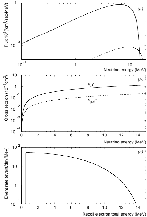
FIG. 4: (a) Input distributions of ^8\text{B} (solid) and hep (dashed) solar neutrino energies. (b) The cross section of the interaction for \nu_e (solid line) and \nu_{\mu,\tau} (dashed line) with electrons as a function of neutrino energy. (c) The spectrum of recoil electrons scattered by ^8\text{B} and hep solar neutrinos.
