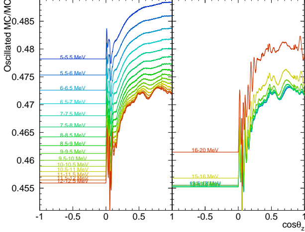
FIG. 53: Predicted solar zenith angle variation assuming a typical LMA solution, \Delta m^2 = 6.3 \times 10^{-5} \text{ eV}^2 and \tan^2 \theta = 0.52 (which is the best fit to the SK energy spectrum, rate, and day/night variation).
