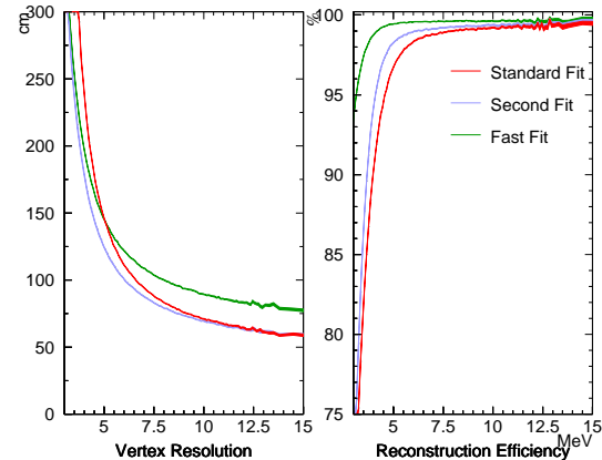
FIG. 11: Vertex resolution (68.2% of reconstructed events reconstruct inside a sphere of radius \sigma from correct vertex) of ^8\text{B} Monte Carlo events as a function of total recoil electron energy. The curves on the right-hand side show the fraction of reconstructed events as a function of total recoil electron energy.
