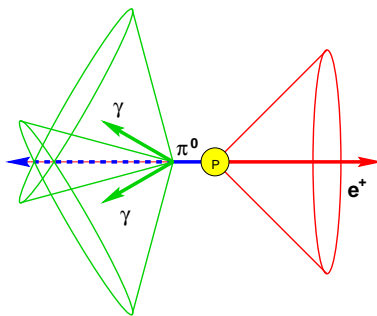
Figure 1: Idealized p \rightarrow e^+\pi^0 decay in Super-Kamiokande [25].
