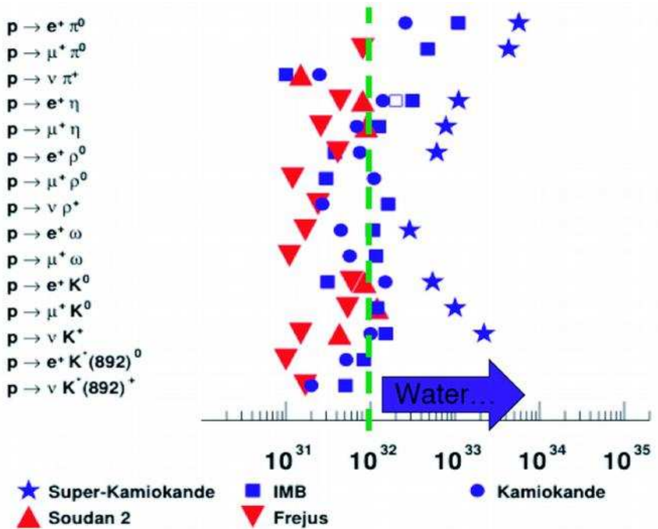
Figure 4: Experimental lower bounds on proton decay partial lifetimes [33]
