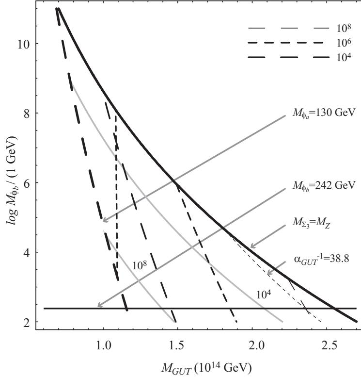
Figure 5: Plot of lines of constant M_{\Sigma_3} and M_{\Phi_a} in the M_{GUT} – \log(M_{\Phi_b}/1 \text{ GeV}) plane, assuming exact one-loop unification. The central values for the gauge couplings as given in the text are used. All the masses are given in GeV units. The triangular region is bounded from the left (below) by the experimental limit on M_{\Phi_a} ( M_{\Phi_b} ). The right bound is M_{\Sigma_3} \geq M_Z . The two grey solid (thick dashed) lines are the lines of constant M_{\Sigma_3} ( M_{\Phi_a} ). The line of constant \alpha_{GUT}^{-1} is also shown. The region to the left of the vertical dashed line is excluded by the proton decay experiments if \alpha = 0.015 \text{ GeV}^3 [212].
