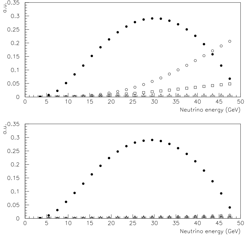
Figure 9: Signal (black circles) and backgrounds for a 1 Kton detector as a function of the neutrino energy at two different baselines: L = 730 km (top panel), L = 3000 km (bottom panel). Background from anti-neutrino induced charm-production (white circles), \tau^+ \rightarrow \mu^+ decays (white triangles) and decay in flight of hadrons in \bar{\nu}_\mu and \nu_e (white squares) neutral-currents interactions are also shown. The signal corresponds to \theta_{13} = 5^\circ and \delta = 90^\circ .
