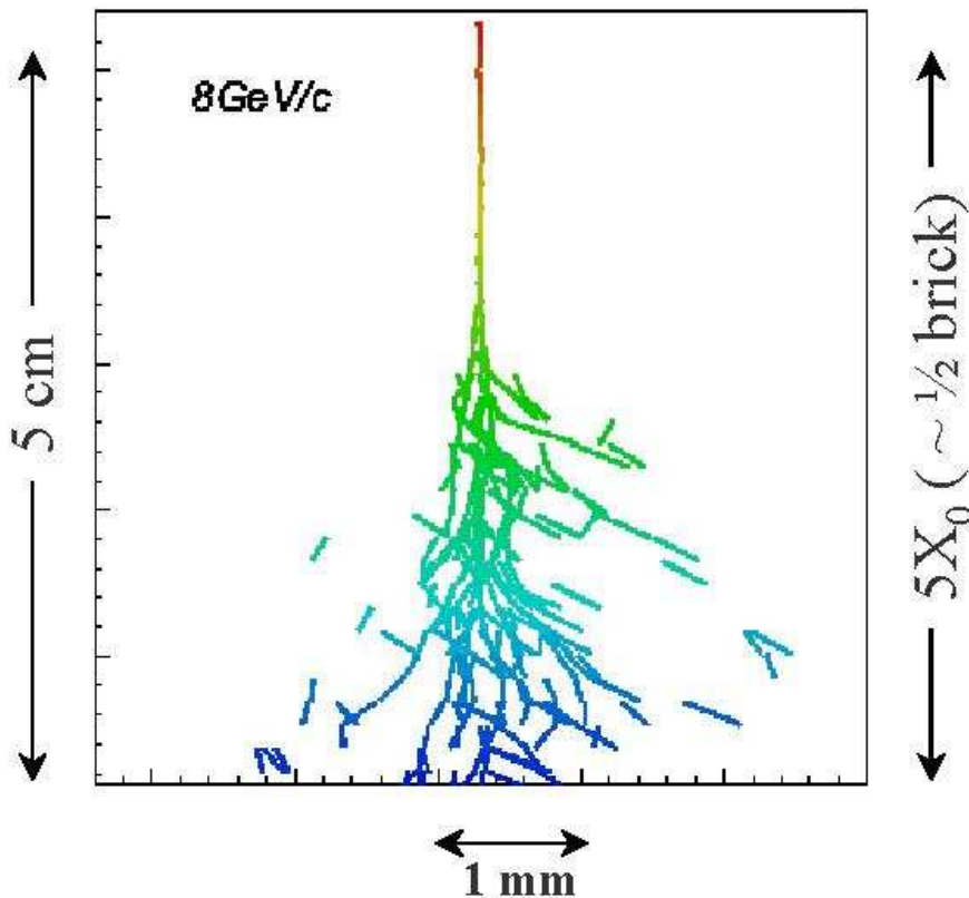
Figure 6: Electromagnetic shower observed in a brick exposed to an electron beam.
