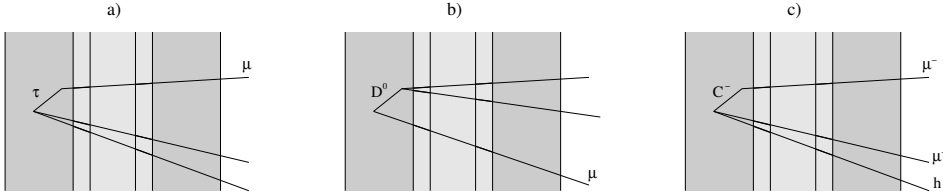
Figure 8: Sketch of signal a) and background b) and c) topologies for \tau \rightarrow \mu decays.
