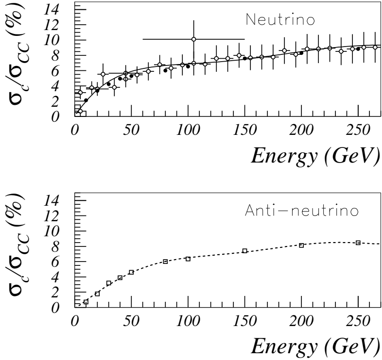
Figure 14: Fraction of neutrino (anti-neutrino) total cross-section that is associated with charm-production. Top: white circles show the average inclusive charm-production cross-section as derived in Ref. [53] and the result of a fit to the data (continuous line); black circles show the predicted cross-section as obtained by a leading-order calculation with m_c = 1.31 GeV [48]. Bottom: white squares show the anti-neutrino induced charm-production as obtained by a leading-order calculation with m_c = 1.31 GeV [48]; the dashed line show a fit to the point.
