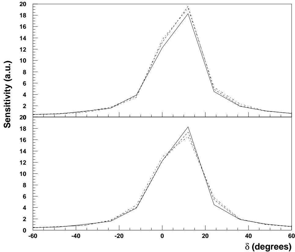
Figure 10: Sensitivity (arbitrary units) of the OPERA-like detector as a function of \delta for \theta_{13} < 2^\circ and different bin configurations. The solid curve is the final choice with four bins. The dashed lines are obtained by changing the bin boundaries (top panel) and by increasing the total number of bins (bottom panel). Signal and background uncertainties are taken into account in the calculation.
