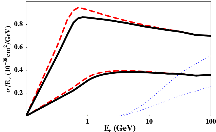
Figure 2: Behaviour of the (anti)neutrino-nucleon cross section as a function of the neutrino energy for \nu_e(\bar{\nu}_e) (long dashed lines), \nu_\mu(\bar{\nu}_\mu) (continuum lines) and \nu_\tau(\bar{\nu}_\tau) (dashed lines) [49].
