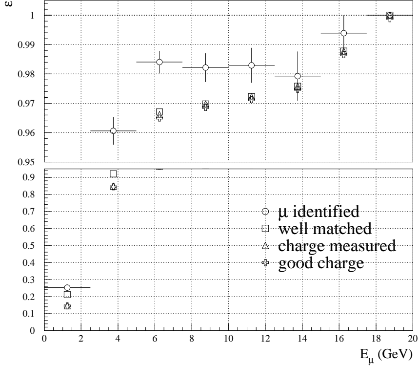
Figure 7: Percentage of \nu_\tau \rightarrow \tau^- X \rightarrow \mu^- \bar{\nu}_\mu \nu_\tau X events with muon identified (dots), well matched to the ECC track (square), reaching the spectrometer (triangle) and with charge correctly assigned (crosses) versus the energy of the muon. To ease the reading, the width of the bins and the statistical errors are shown just for the first mark.
