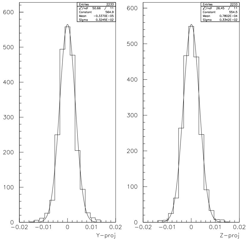
Figure 4: The measured angular resolution routinely achieved with an ECC shown for both angular projections.
