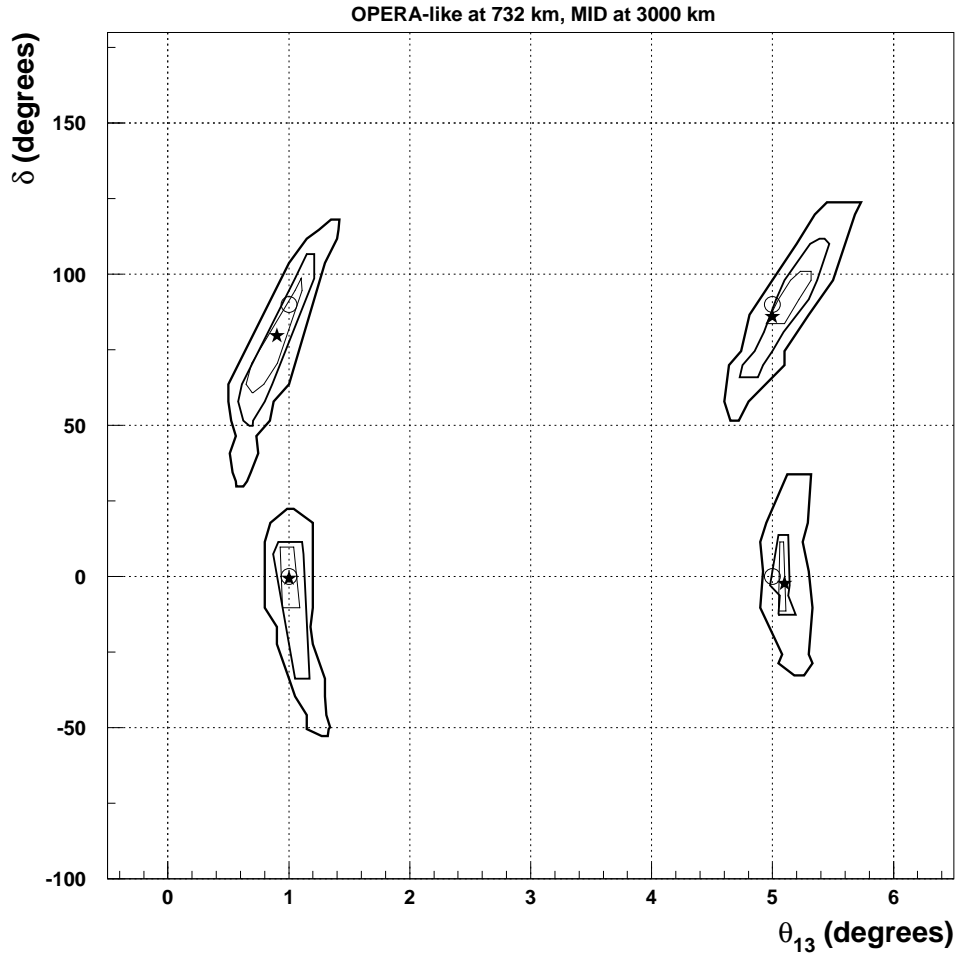
Figure 11: Expected 68.27%, 90% and 99% confidence regions in the (\theta_{13}, \delta) plane corresponding to four simulated points. Both an OPERA-like detector at 732 km and an iron detector at 3000 km are combined. The stars denote the best fit points, while the open circles are the true simulated points.
