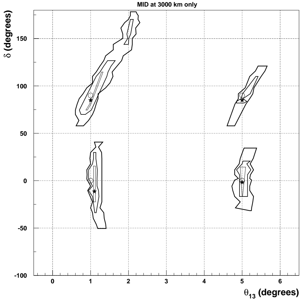
Figure 13: Expected 68.27%, 90% and 99% confidence regions in the (\theta_{13}, \delta) plane corresponding to four simulated points. Only an iron detector at 3000 km is considered, with two beam polarities. The stars denote the best fit points, while the open circles are the true simulated points.
