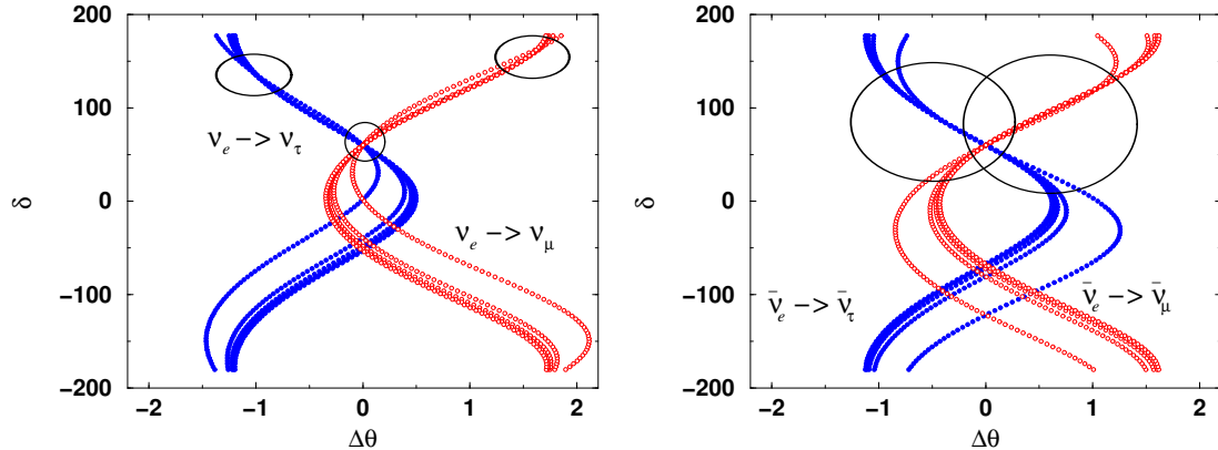
Figure 1: Equiprobability curves in the (\Delta\theta, \delta) plane, for \bar{\theta}_{13} = 5^\circ, \bar{\delta} = 60^\circ, E_\nu \in [5, 50] GeV and L = 732 km for the \nu_e \rightarrow \nu_\mu and \nu_e \rightarrow \nu_\tau oscillation (neutrinos on the left, anti-neutrinos on the right). \Delta\theta is defined as the difference between the reconstructed parameter \theta_{13} and the input parameter \bar{\theta}_{13} , \Delta\theta = \theta_{13} - \bar{\theta}_{13} .
