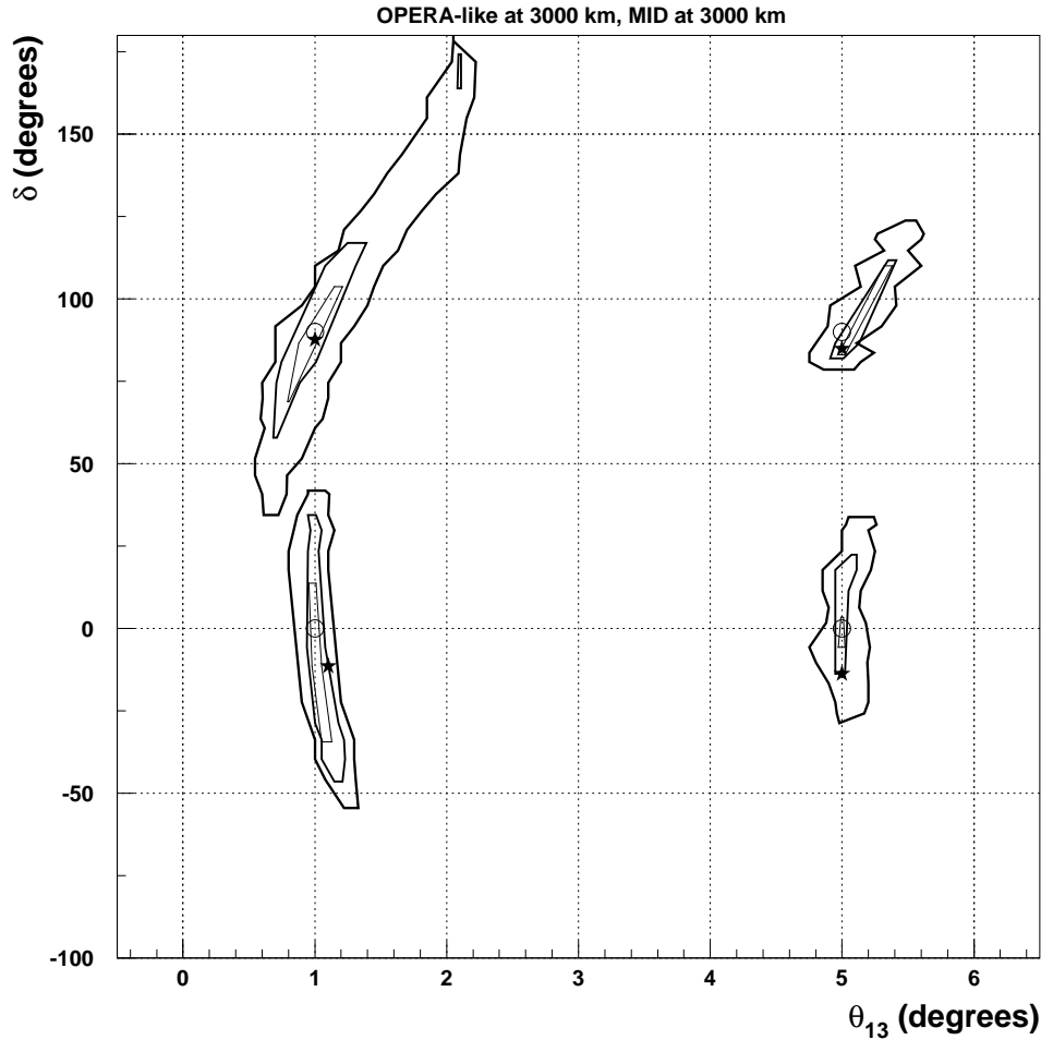
Figure 12: Expected 68.27%, 90% and 99% confidence regions in the (\theta_{13}, \delta) plane corresponding to four simulated points. Both an OPERA-like detector at 3000 km and an iron detector at 3000 km are combined. The stars denote the best fit points, while the open circles are the true simulated points.
