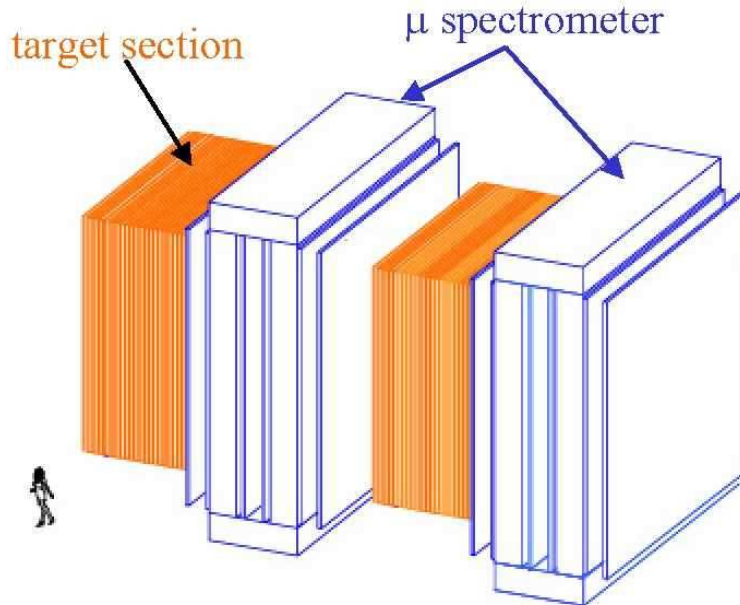
Figure 3: OPERA at CNGS.
