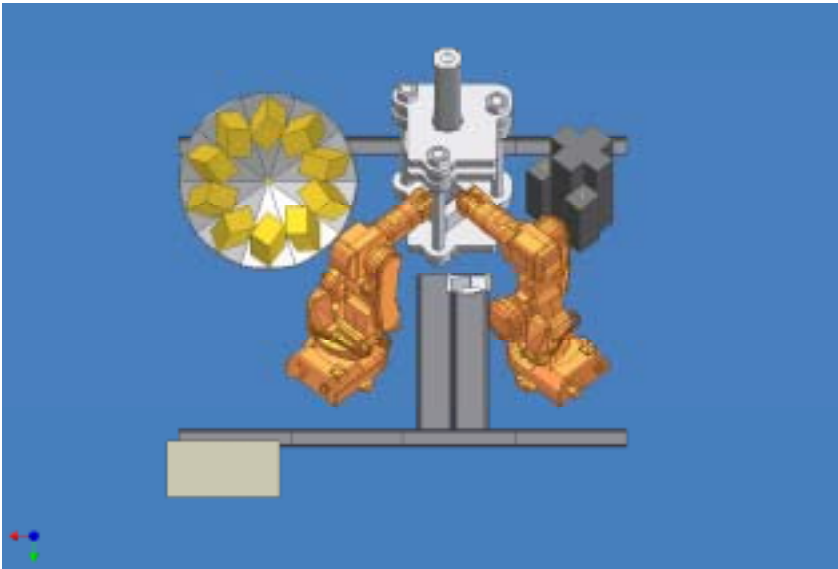
Fig 6 Final piling-pressing station layout.
