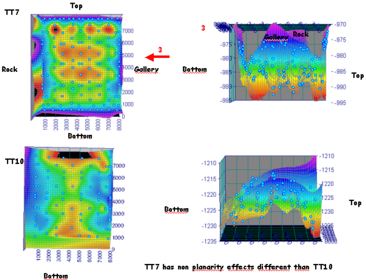
Fig.5: 3D representation of clouds of points measured with Photogrammetry on the surface of two target tracker modules
