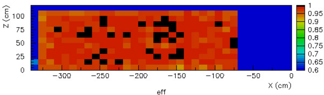
Preliminary efficiency map of a glass RPC
