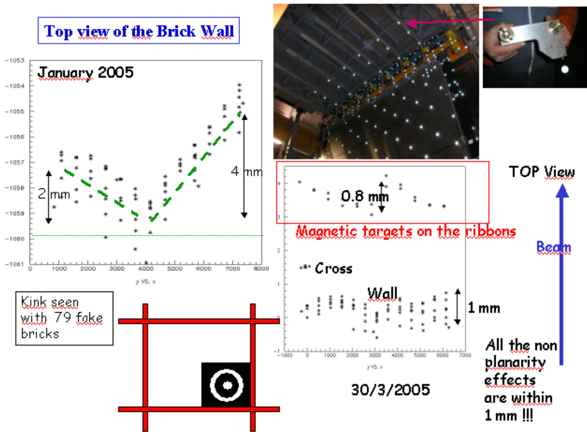
Fig.4: Top views of the cloud of points measured on a wall before (Left) and after (Right) having fixed the alignment interference with the TT. The final dispersion along the beam axis of the points on a wall is better than 1 mm.
