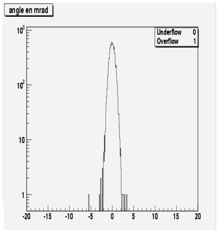
Silicon telescope put after the magnetic spectrometer
