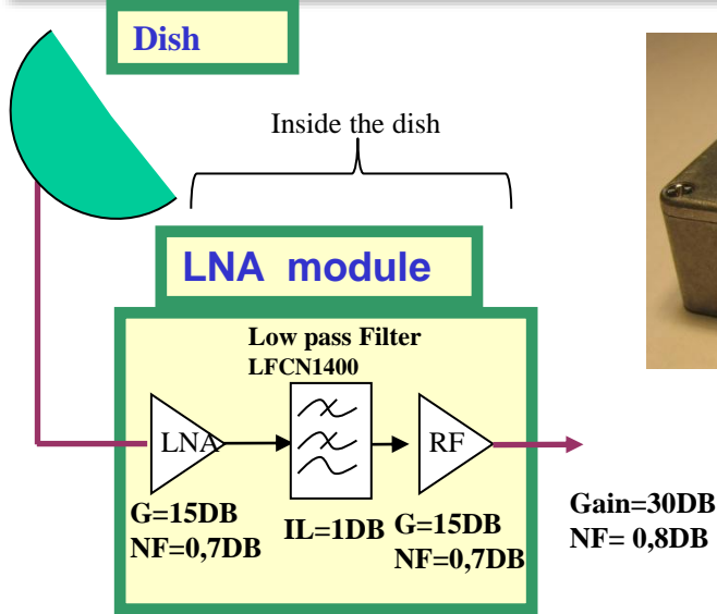
Gain(F) LNA_Parabole
