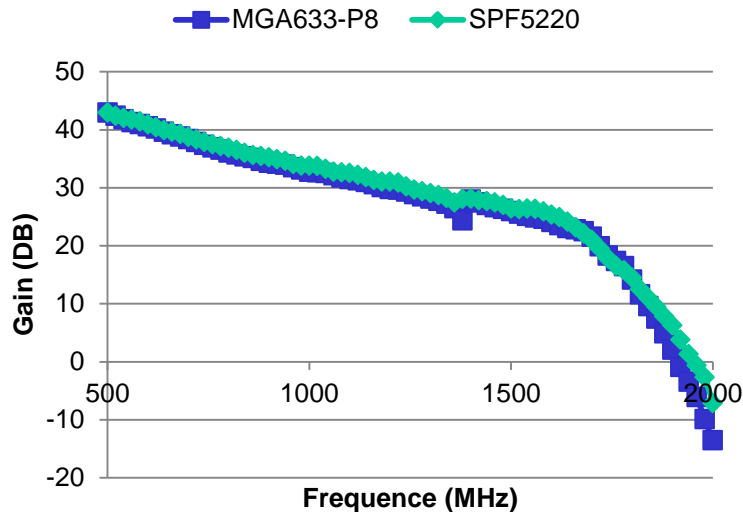
Gain(F) LNA_Parabole
