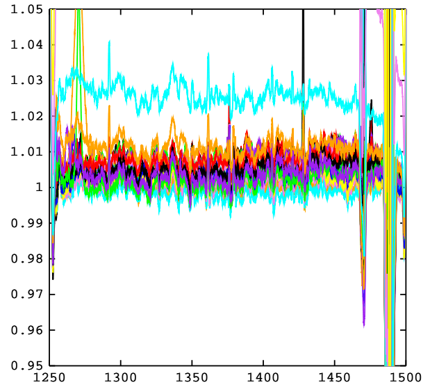
Abell185/20110806 Raw: On Ch 1
