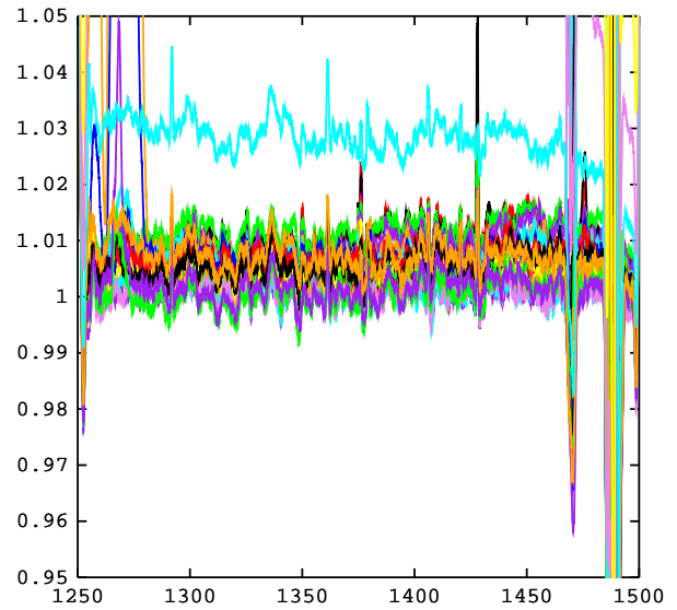
Abell185/20110806 Raw: Off Ch 1
