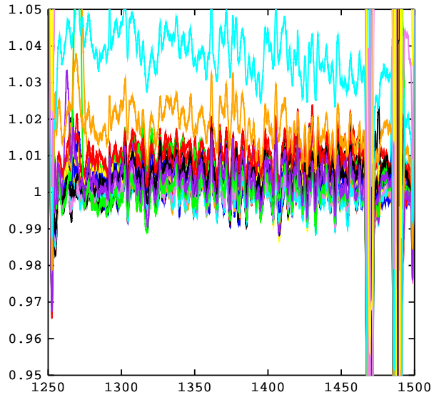
Abell185/20110806 Raw: On Ch 0
