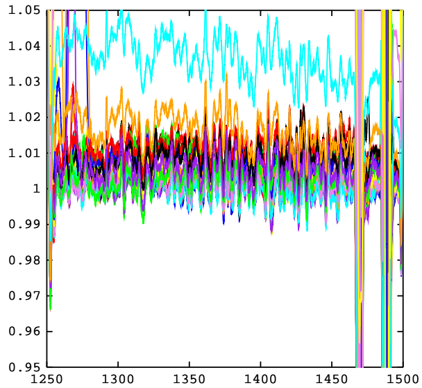
Abell185/20110806 Raw: Off Ch 0
