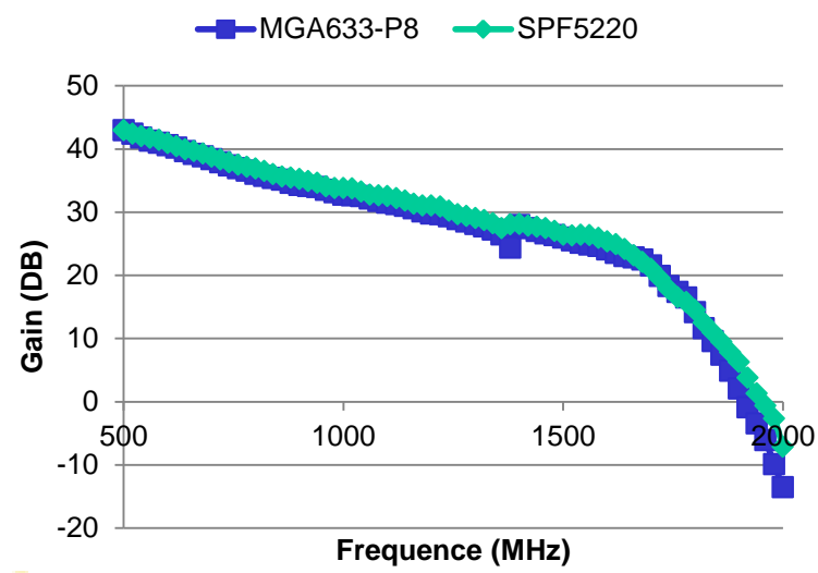
Gain(F) LNA_Parabole
