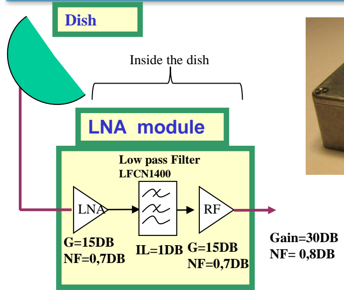
Gain(F) LNA_Parabole
